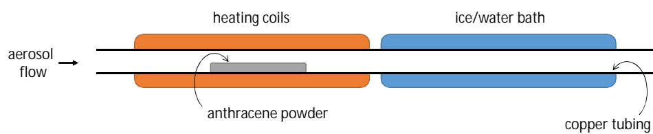
Coating apparatus #1
