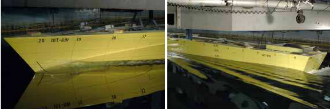
Figure 7: Photographs of Model During Testing
