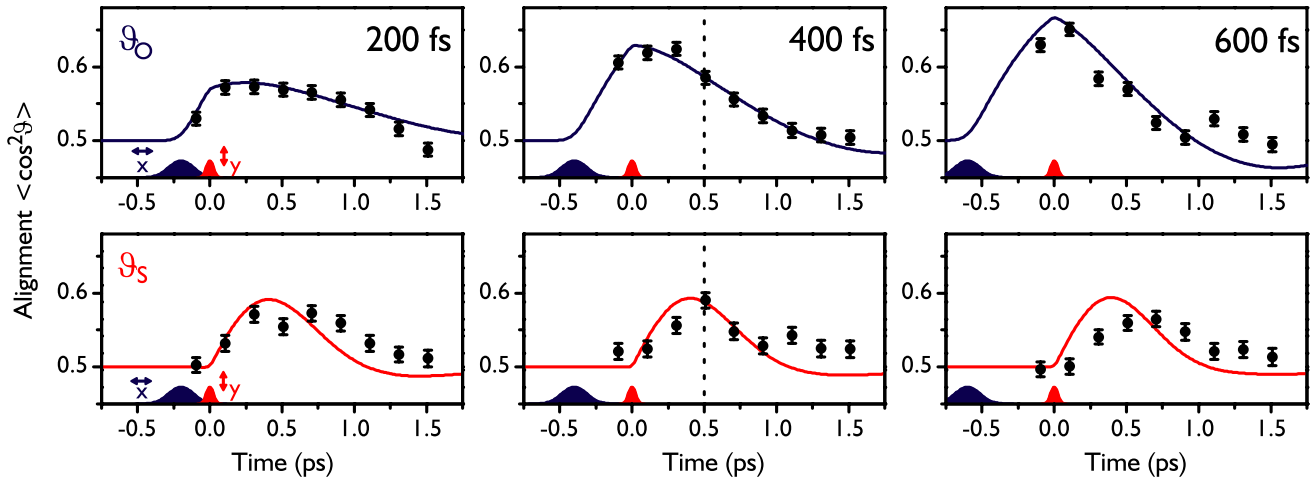
FIG. 3 (color online). Measured time dependence of \text{SO}_2 molecular axis alignment. The three columns show data for pulse separations of 200 fs (left), 400 fs (middle), and 600 fs (right). The zero of time is defined by the peak of the second laser pulse. Experimental data points are shown in black with error bars corresponding to the standard error of the mean. The solid lines are the results of classical calculations. The dashed line shows the maximum FF3DA achieved.
