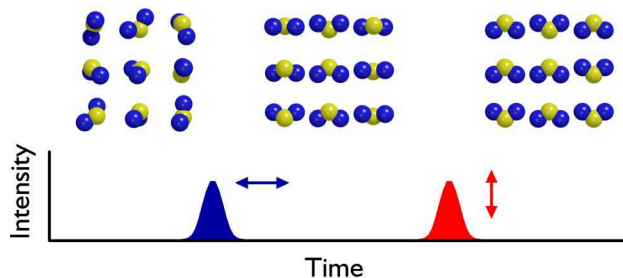
FIG. 1 (color online). Scheme for field-free 3D alignment of \text{SO}_2 molecules using time-separated laser fields. S atoms are shown in yellow and O atoms are shown in blue. For details see text.
