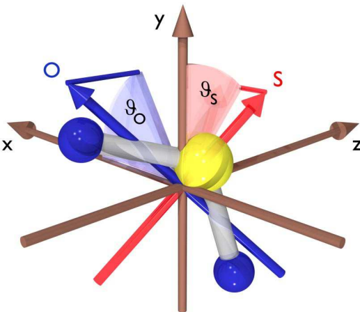
FIG. 2 (color online). Definition of angles \vartheta_O and \vartheta_S . The laboratory frame is defined by the propagation direction of the laser pulses (the z axis) and the polarization directions of the two linearly polarized alignment pulses; the first pulse is polarized along the x axis, the second along the y axis.
