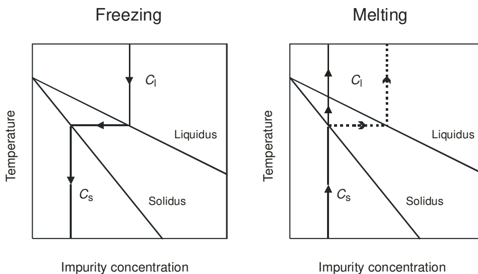
Figure 1: Simplified schematic representation of freezing (on the left) and melting (on the right) in a binary phase diagram for an impurity with k_0^i < 1 at low concentrations. For macroscopic phase changes, only the way along the solid lines is allowed. The dotted melting line is possible in microscopic regions.
