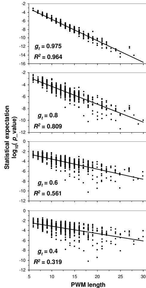
Fig. 2. p -value of 585 vertebrate PWMs over various G values. The length factor (L-w+1) has not been incorporated into these p -values. For a sequence of length L , these p -values have to multiply the values by a factor of L-w+1 .
