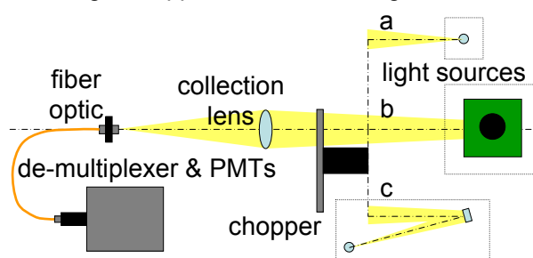
Figure 1: Calibration setup a.) strip filament lamp, b.) integrating sphere, and c.) irradiance standard
