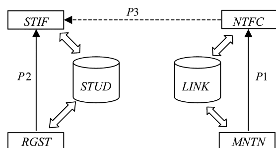
Fig. 1 A conversation schemata for course maintenance
