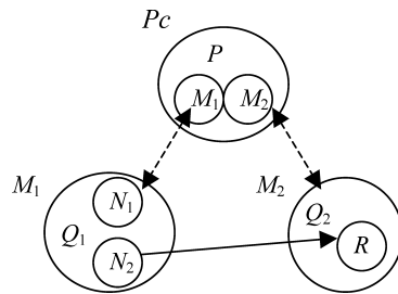
Fig. 2 Software architecture for the producer-consumer program
