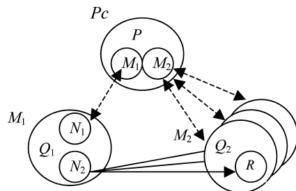
Fig. 3 Software architecture for the producer-multi-consumer program
