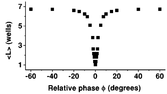
FIG. 3. Phase control of the Floquet states' localization length in an ( N=10 )-well system with random couplings: \Omega_n=0.5(1+\alpha)\Omega ; \alpha is random between 0 and 1. V_0/\omega=2.48 ; \Omega/\omega=1/4 .
