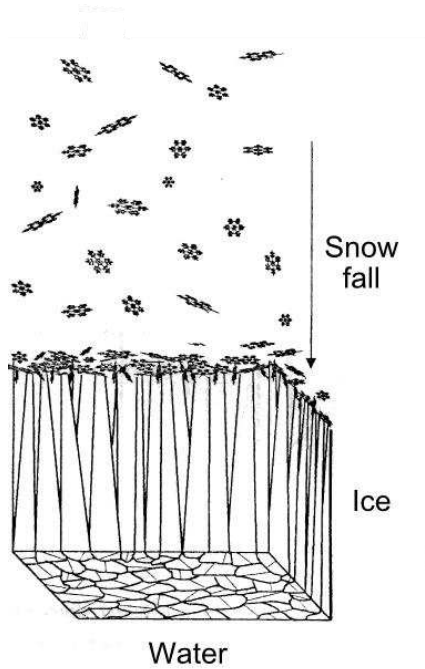
Figure 1: A common scenario for the initiation and downward growth of an ice cover. That ice is typically clear ice.
