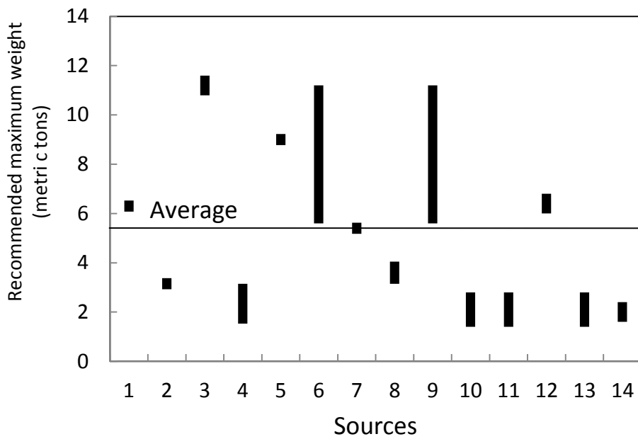
Figure 8: Recommendations from various sources, assuming a total ice thickness of 40 cm made of clear ice and natural white ice in equal proportion and of questionable quality.
