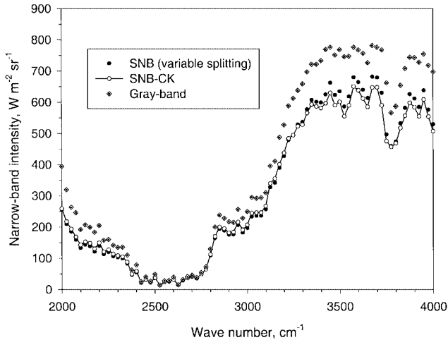
Fig. 2 Comparisons of narrowband integrated radiation intensities at (1 m, 1 m, 7.9 m) and along the direction (0.0990147, 0.0990147, 0.990147) for the isothermal case with scattering. Particle number density is 2 \times 10^9 \text{ m}^{-3} .
