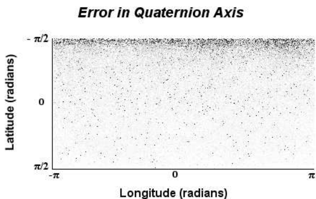
Figure 9: Analysis of error on quaternion axis.
