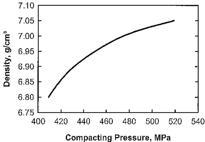
Figure 10. Effect of compacting pressure on the density of 20 mm thick stator segments.
