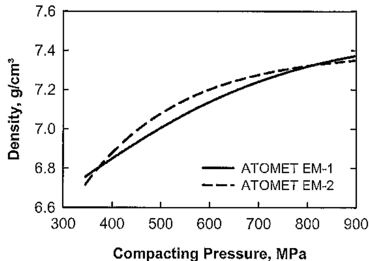
Figure 4. Effect of compacting pressure on the density of TR bars pressed from two SMC materials.
