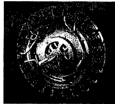
Figure 13. Final SMC stator comprising four segments inserted between two aluminium flanges.
