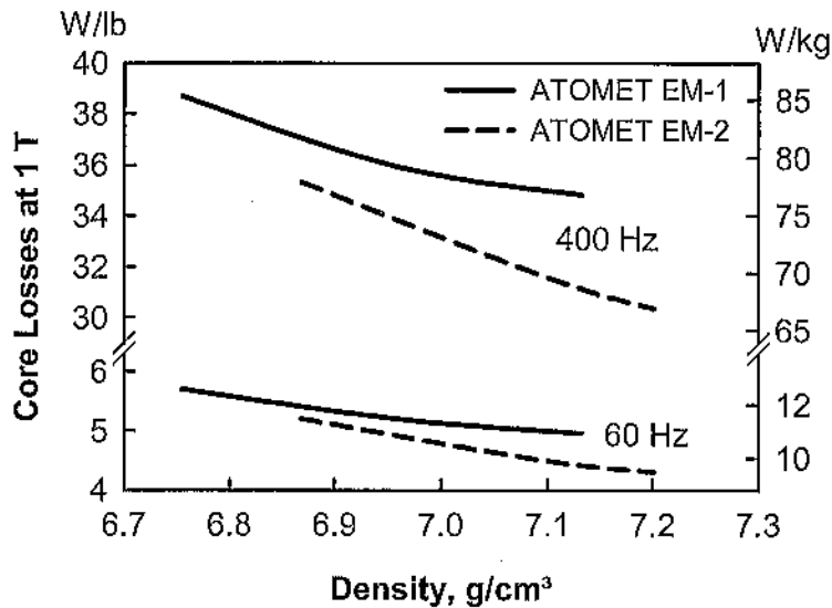
Figure 7. Effect of density on the total core losses at 1 Tesla measured at 60 and 400 Hz.
