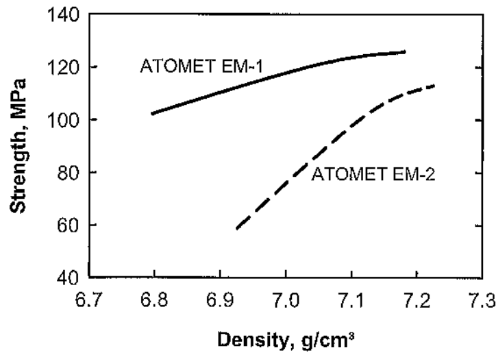
Figure 5. Effect of density on the mechanical strength of TR bars pressed from two SMC materials.
