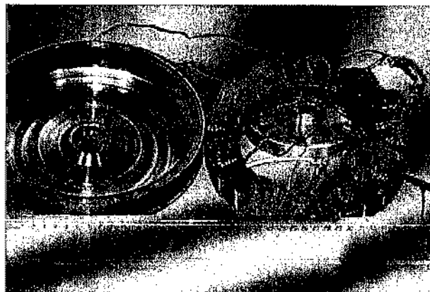
Figure 3. First prototype with the rotor (left) and machined SMC stator (right).
