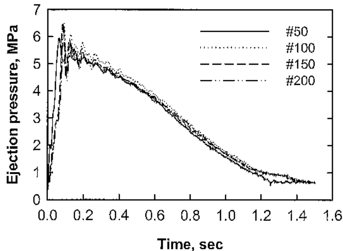
Figure 12. Ejection curves taken during the production of 20 mm thick stator segments pressed to 6.85 g/cm 3 (5 parts/min).
