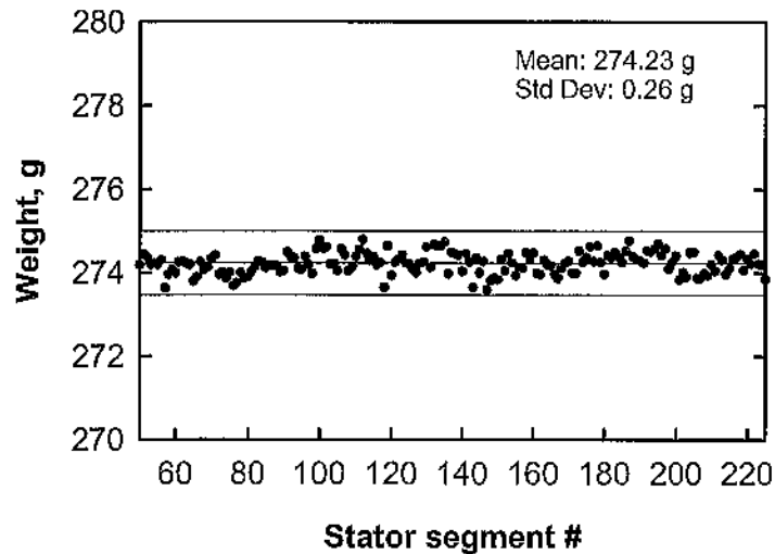
Figure 11. Weight variation of the stator segments (lines stand for the mean \pm 3 std dev).
