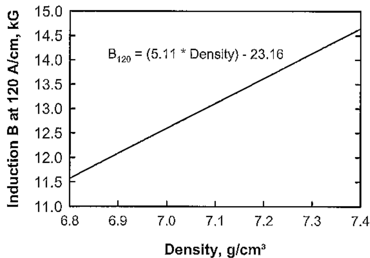
Figure 6. Effect of density of SMC materials on the magnetic induction at an applied field of 120 A/cm.
