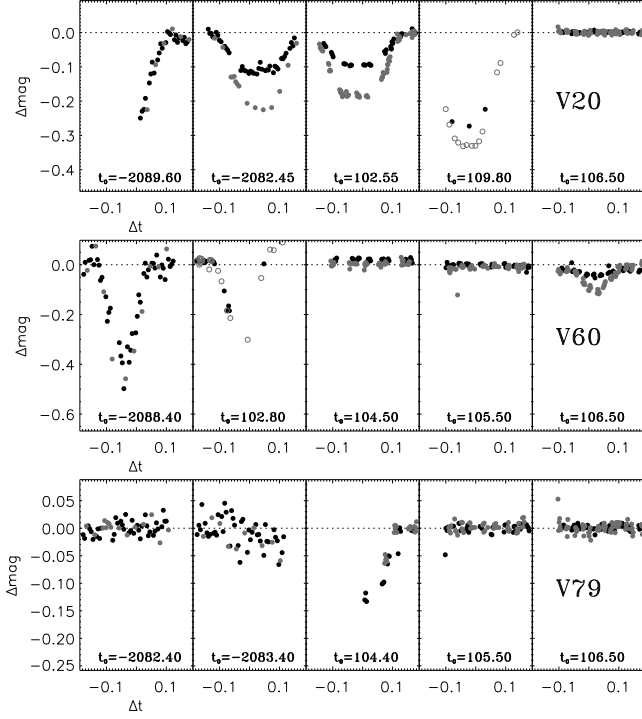
Fig. 9. Light curves of three eclipsing binary stars. The time corresponding to 0.0 on the abscissa is HJD – 2452 000 and is given at the bottom of each panel as t_0 . One or more nights without eclipses are shown for comparison. Black and grey symbols are V and I measurements, while the open circles are R measurements from MOCH01 .
