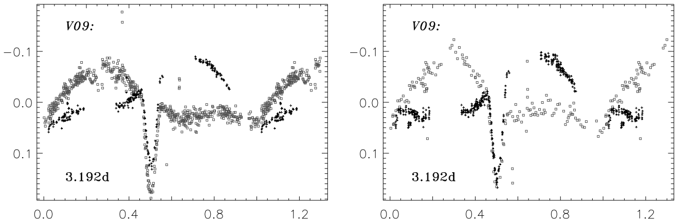
Fig. 8. Phased light of the RS CV-type variable V9 in NGC 6791 in the V (left plot) and I filter (right plot). The black + symbols are data from NOT01 while the grey symbols are from either SMR95 (box symbol) or MOCH01 (filled grey symbols) The MOCH01 data are not plotted in the right plot since Mochejska et al. (2002) did not observe in I .
