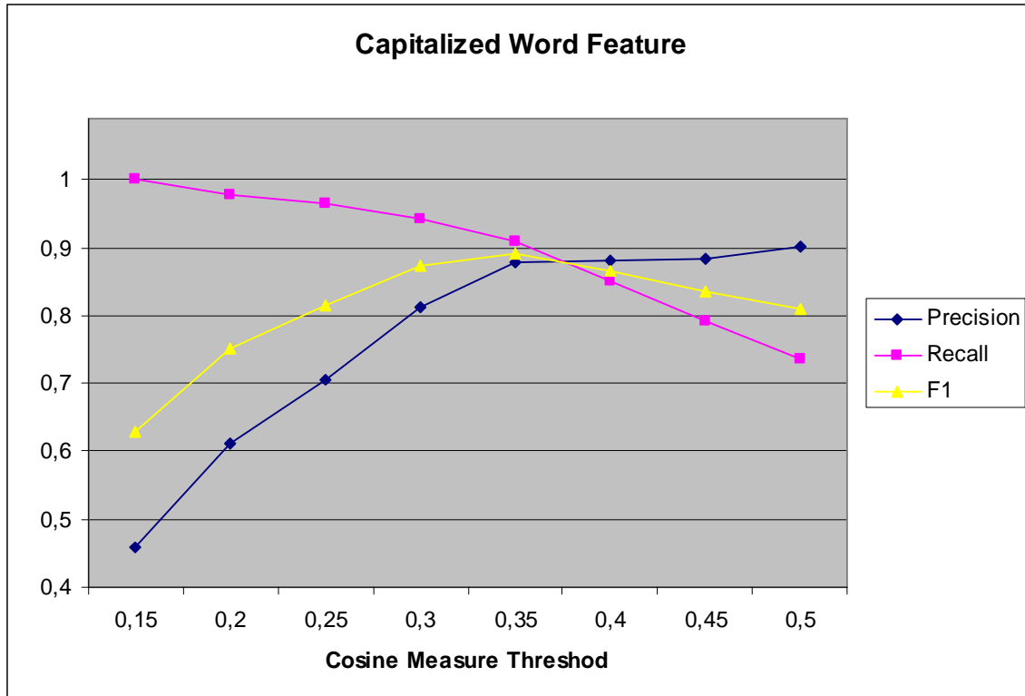
Figure 2: Capitalized Word Feature Precision and Recall
