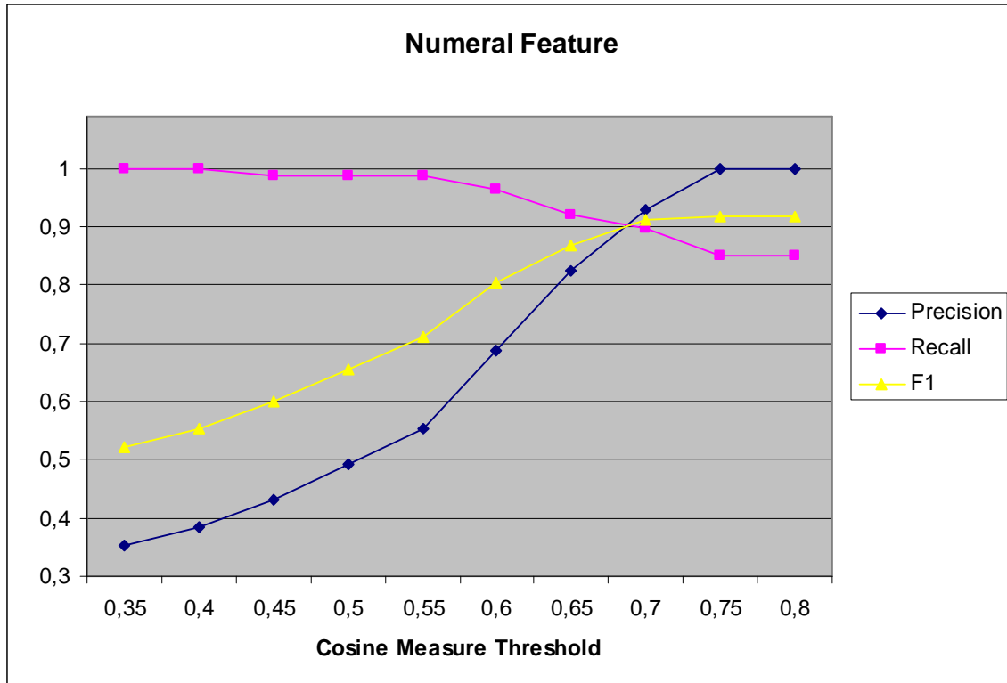
Figure 1: Numeral Feature Precision and Recall
