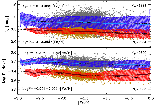
Figure 9. Top: Visual amplitude as function of iron abundance for RRAb (grey dots) and RRc (dark yellow dots). The blue and the red solid lines display the running averages for RRAb and RRc variables and the shaded areas show the corresponding standard deviation. The dot-dashed lines display the linear regressions and their coefficients are labelled. Bottom: Same as the top, but with the \log P on the y-axis.
