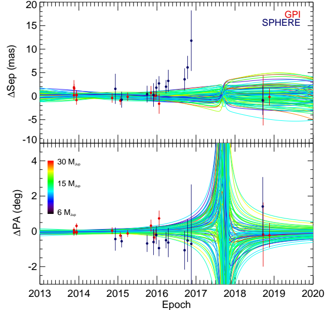
Figure 13. Comparison of the GPI and SPHERE astrometry between 2013 and 2020, with the lowest \chi^2 orbit subtracted off (Case 3). We find no evidence for a systematic offset in plate scale ( 1.001 \pm 0.003 ), but significant evidence of a position angle offset of -0.47 \pm 0.14^\circ .
