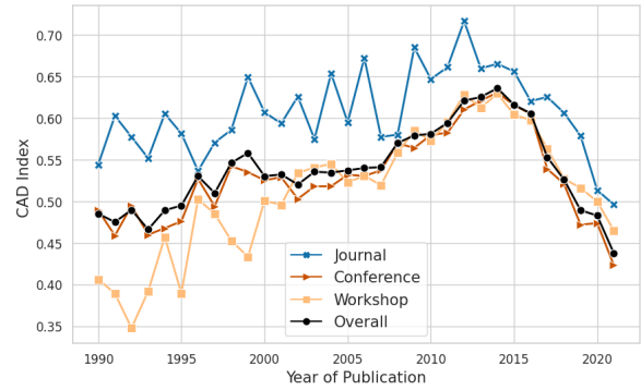
Figure 4: Citation Age Diversity (CAD) Index across years.
