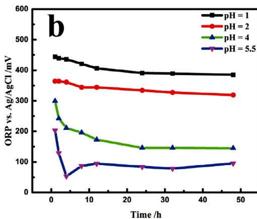
Fig. 5. (a) pH and (b) ORP during calcine oxidative leaching (see Table S1 for test conditions).
