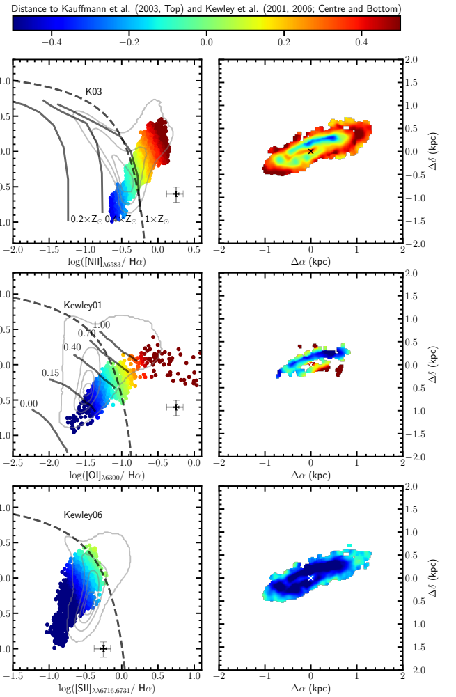
Fig. 12. Same as Fig. 11 for the galaxy NGC 4526.
