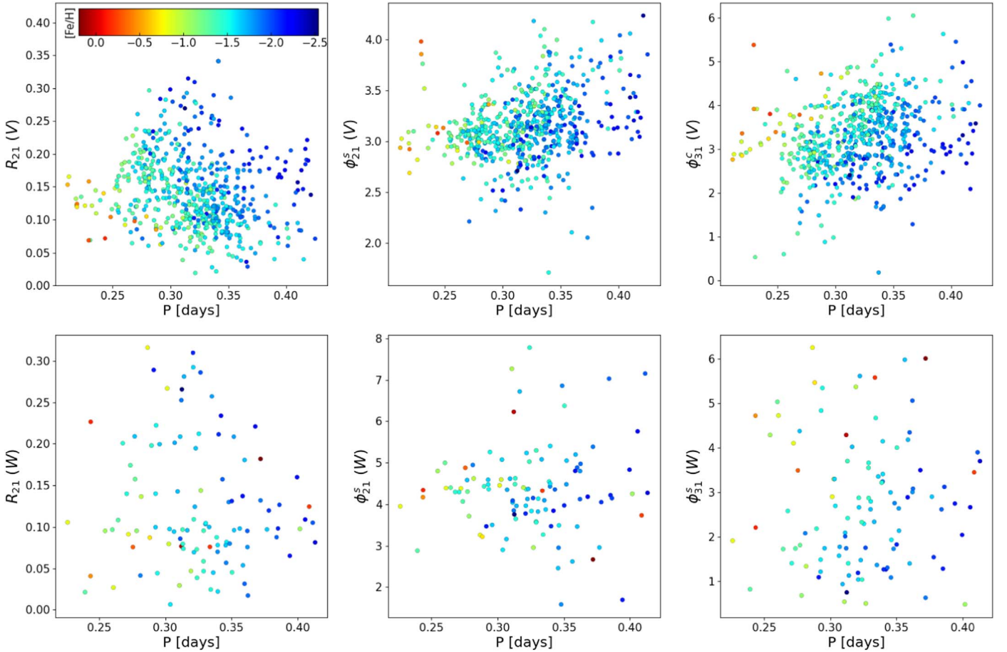
Figure 4. ASAS-SN V -band (top row) and WI -band (bottom row) Fourier parameters as functions of the period. RRLs are color-coded based on their spectroscopic calibration metallicities. In the rightmost column ( \phi_{31} ), [\text{Fe}/\text{H}] generally goes from metal-rich in the left (red) to metal-poor in the right (blue). All parameters have been derived with a sine Fourier decomposition (indicated with a s superscript), except for the top right panel ( \phi_{31}^c(V) values) where the Fourier phase parameters have been converted into a cosine decomposition (see text). Average errors for each of the parameters plotted are smaller than the size of the data points.
