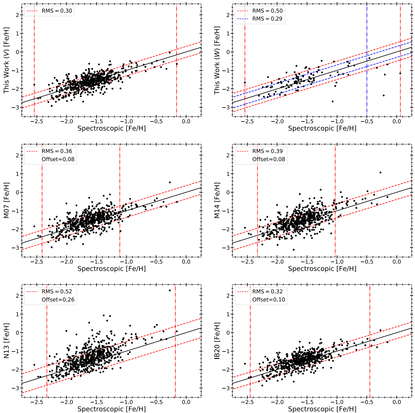
Figure 8. Comparison of the spectroscopic [\text{Fe}/\text{H}] abundances of our calibration sample and those derived with a variety of photometric metallicities, such as those presented in Section 3.1 (top row), M07 and M14 (middle row), and N13 and IB20 (bottom row). The diagonal dashed lines represent the rms dispersion about the ideal one-to-one relation. The metallicity range used to calibrate each relation is indicated by the two vertical dash-dotted red lines. An additional rms is shown for the WISE band relation (top right panel, dashed blue lines), calculated using only the stars with [\text{Fe}/\text{H}] \lesssim -0.5 (vertical dash-dotted blue line).
