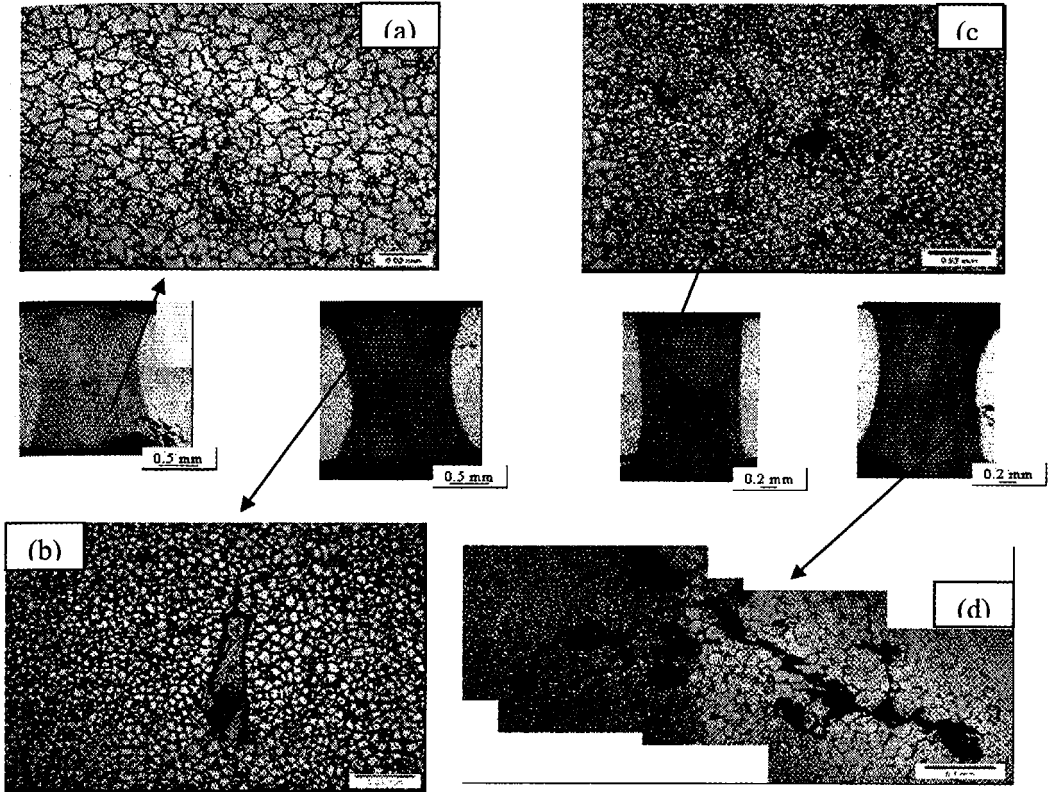
Figure 7 – Solidification Cracks in the FZ initiated by Various Sources Observed in Laser Welding of ZE41A-T5 Mg alloy
