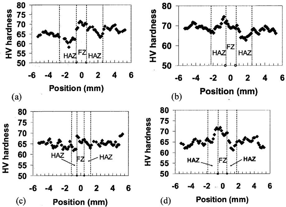
Figure 9 – Vickers Microindentation Hardness for Welding Speed at (a) 4, (b) 5, (c) 6, and (d) 7 m/min
