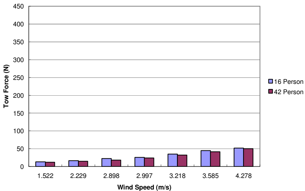
Figure 6.3: Mean tow loads for the full scale 16 and 42 person life rafts across varying wind speeds.
