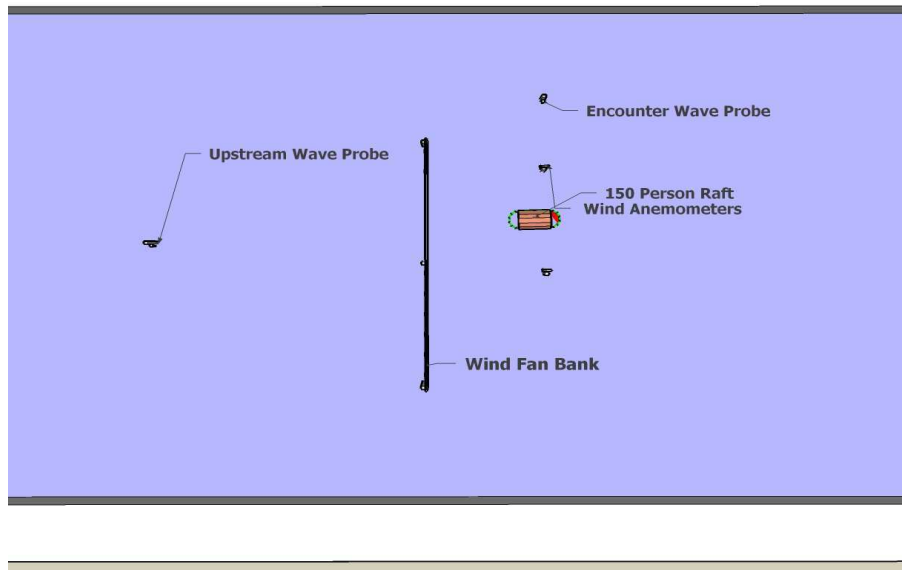
Figure 5.2: Overhead view of OEB setup (150 person model scale life raft pictured)
