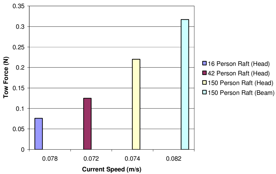
Figure 6.7: Tow force generated by each of the model scale rafts in varying current speeds.
