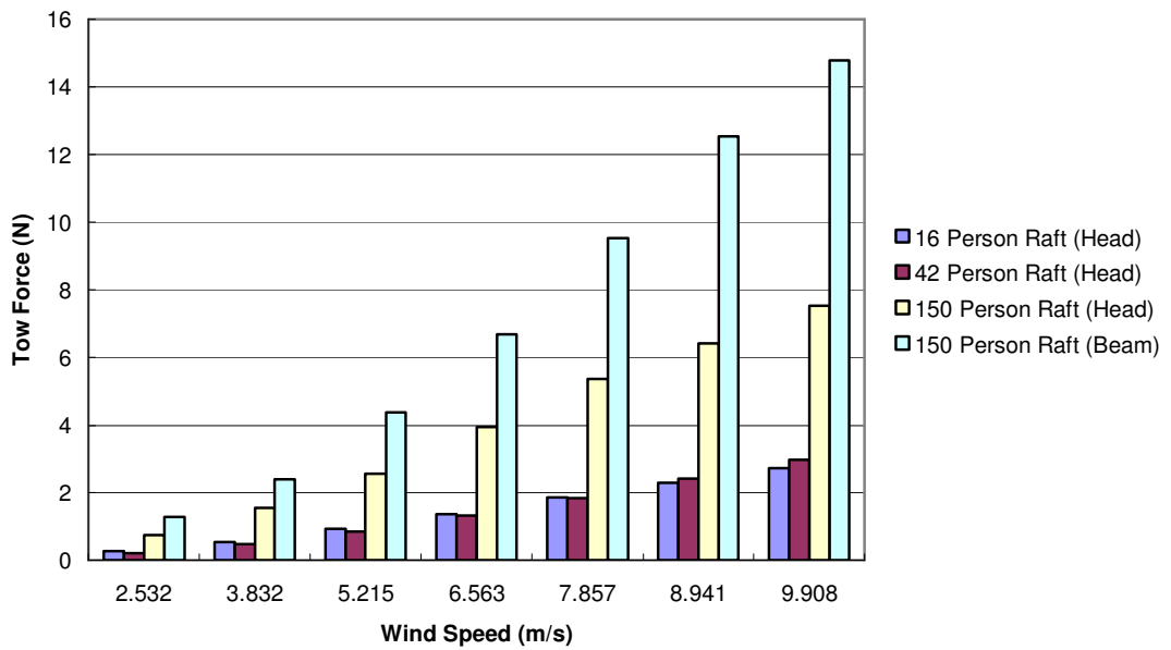
Figure 6.4: Mean tow loads for the full scale 150 person life raft, head and beam on to the wind field, across varying wind speeds
