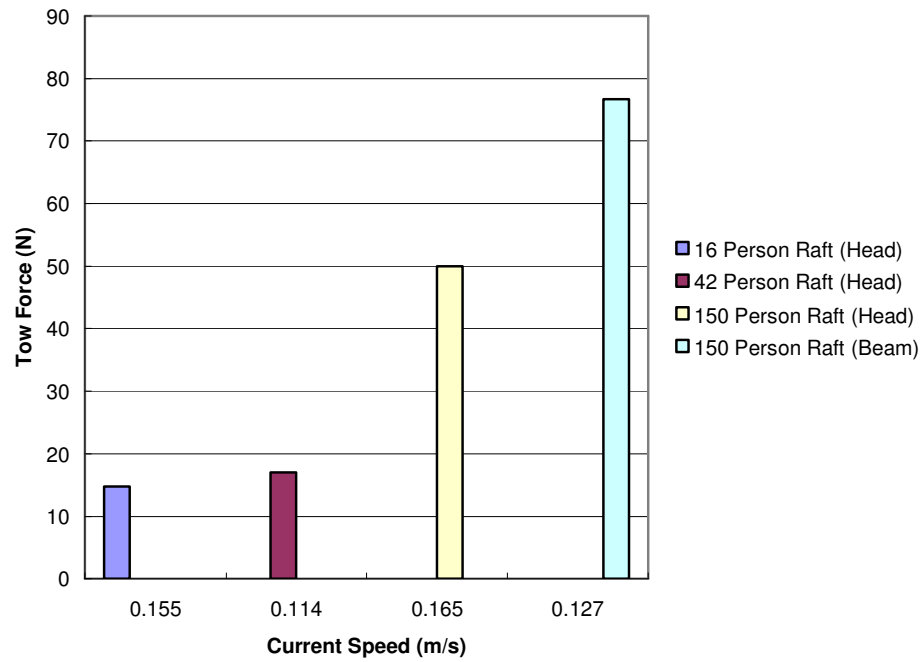
Figure 6.6: Tow force generated by each of the full scale rafts in varying current speeds.
