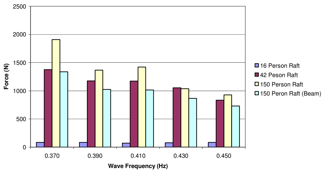
Figure 6.1: Mean tow force plus 2 standard deviations for full scale life rafts across varying wave frequencies.
