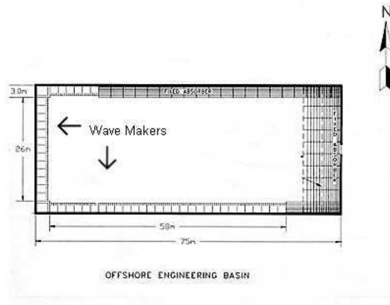
Figure 3.1: Drawing of Institute for Ocean Technology's Offshore Engineering Basin (all distances in meters).
