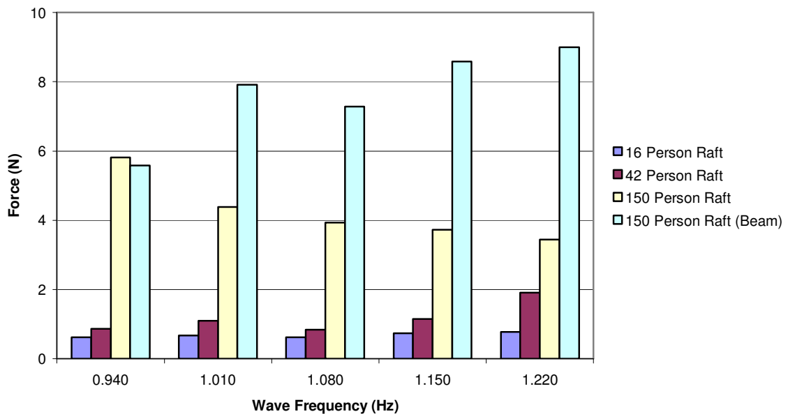
Figure 6.2: Mean tow force plus 2 standard deviations for model scale life rafts across varying wave frequencies
