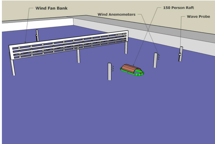
Figure 5.1: OEB setup (150 person model scale life raft pictured).
