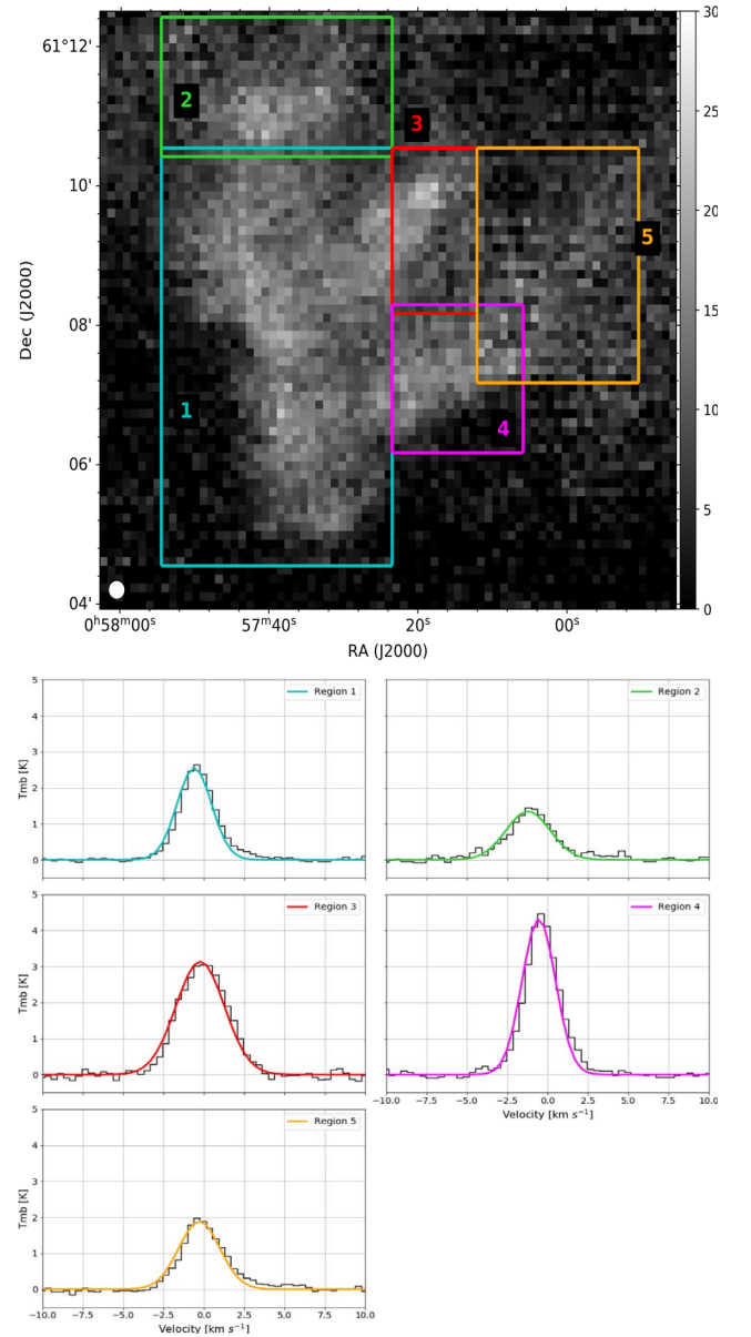
Figure 11. Same as Figure 10 but for five regions in IC 59 and with extracted spectra filled in gray. The fit parameters for each Gaussian are shown in Table 2.
