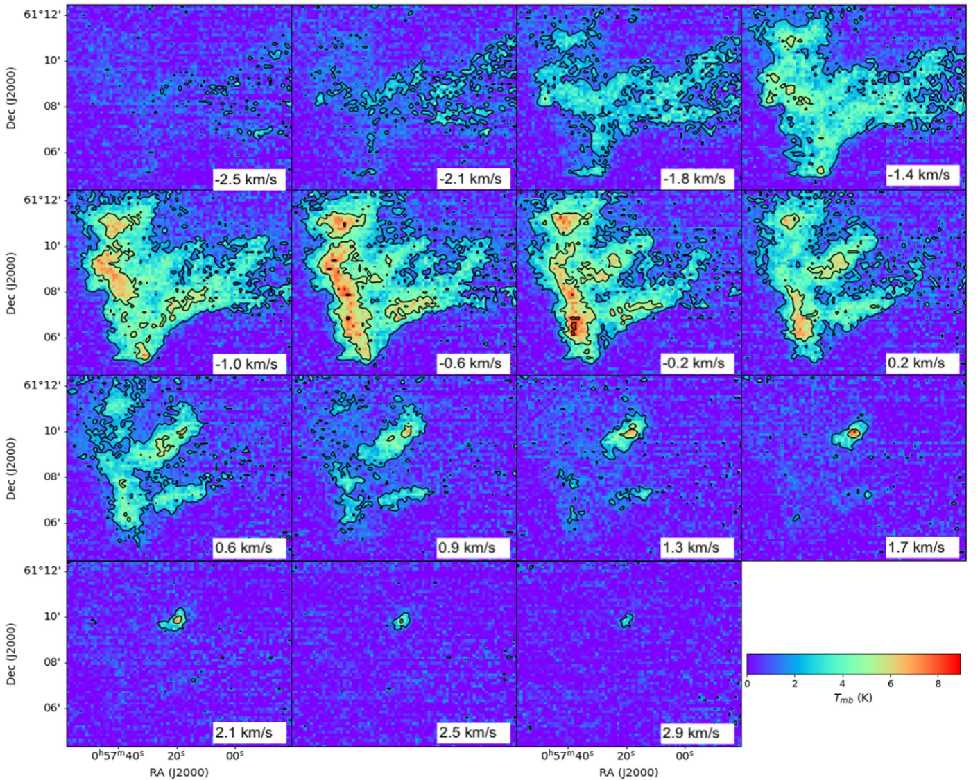
Figure 7. Same as Figure 6 but for IC 59.
