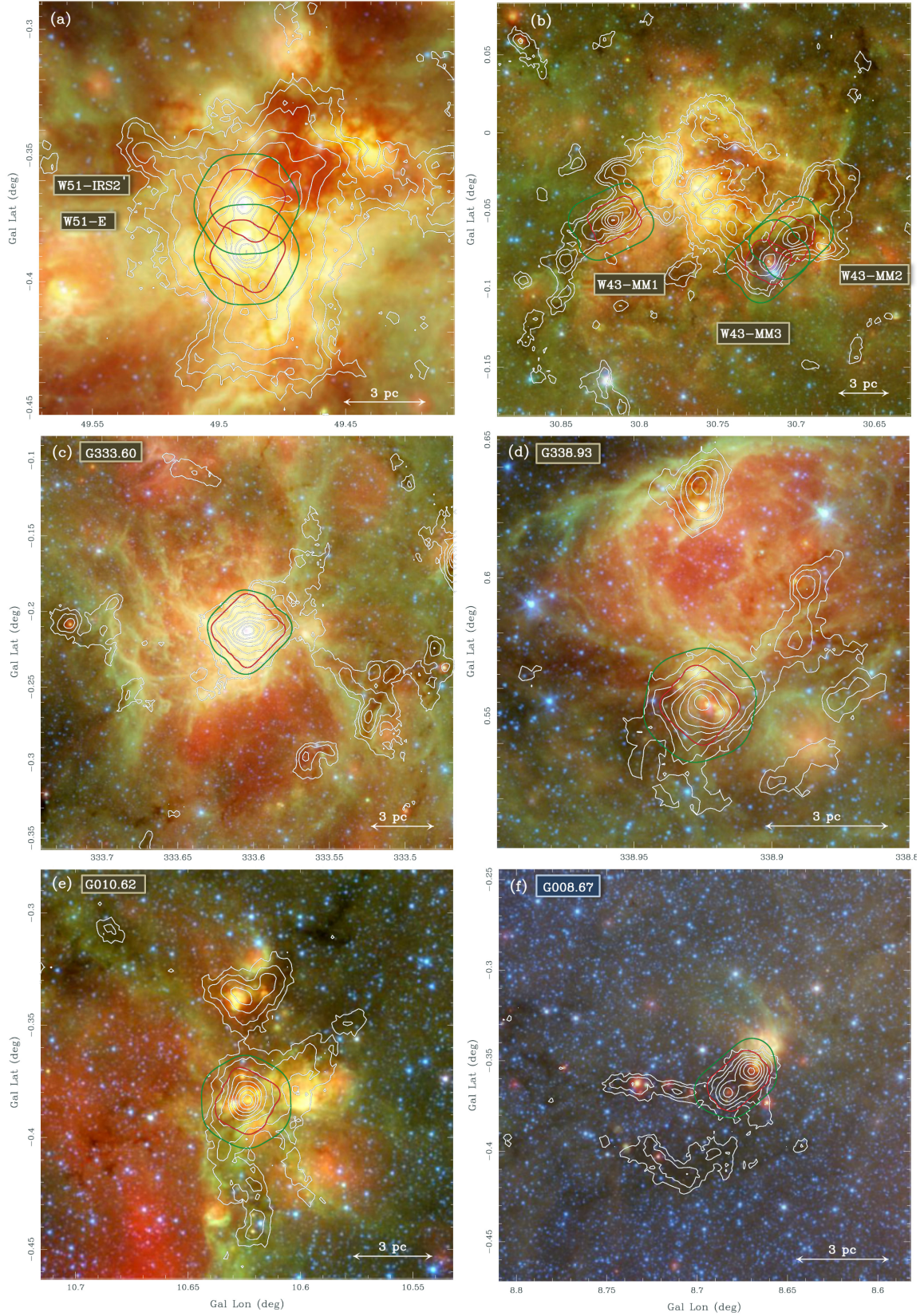
Fig. 1. Overview of the surroundings of the ALMA-IMF protocluster clouds, ordered by decreasing mass of their central clump (Col. (9) of Table 1): W51-E and W51-IRS2 (panel a), W43-MM1, W43-MM2, and W43-MM3 (panel b), G333.60 (panel c), G338.93 (panel d), G010.62 (panel e), and G008.67 (panel f). ATLASGAL 870 μm emission contours (logarithmically spaced from 0.45 Jy beam -1 to 140 Jy beam -1 with a 19.2'' beam) are overlaid on Spitzer three-color images (red represents MIPS 24 μm, green GLIMPSE 8 μm, and blue GLIMPSE 3.6 μm). The green and red contours outline the primary beam response of the ALMA 12 m array mosaics down to 15% at 3 mm and 1.3 mm, respectively. A 3 pc scale bar is shown in the lower-right corner of each image.
