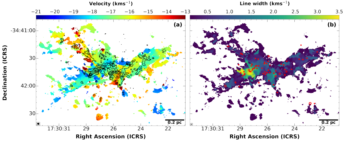
Fig. 7. Network of filaments, which interact at the center of the G353.41 protocluster. First-moment ( panel a ) and second-moment ( panel b ) 12 m array images of the \text{N}_2\text{H}^+(1-0) isolated hyperfine satellite, corresponding to the centroid velocity and line width, respectively. The 1.3 mm continuum emission is overlaid in (a) in black contours, which are 4, 20, 40, 80, and 160 in units of \sigma = 0.3 \text{ mJy beam}^{-1} . Red ellipses in b denote the ALMA-IMF core locations. Ellipses in the lower-left corners represent the angular resolutions of the \text{N}_2\text{H}^+(1-0) in a and 1.3 mm continuum images in b.
