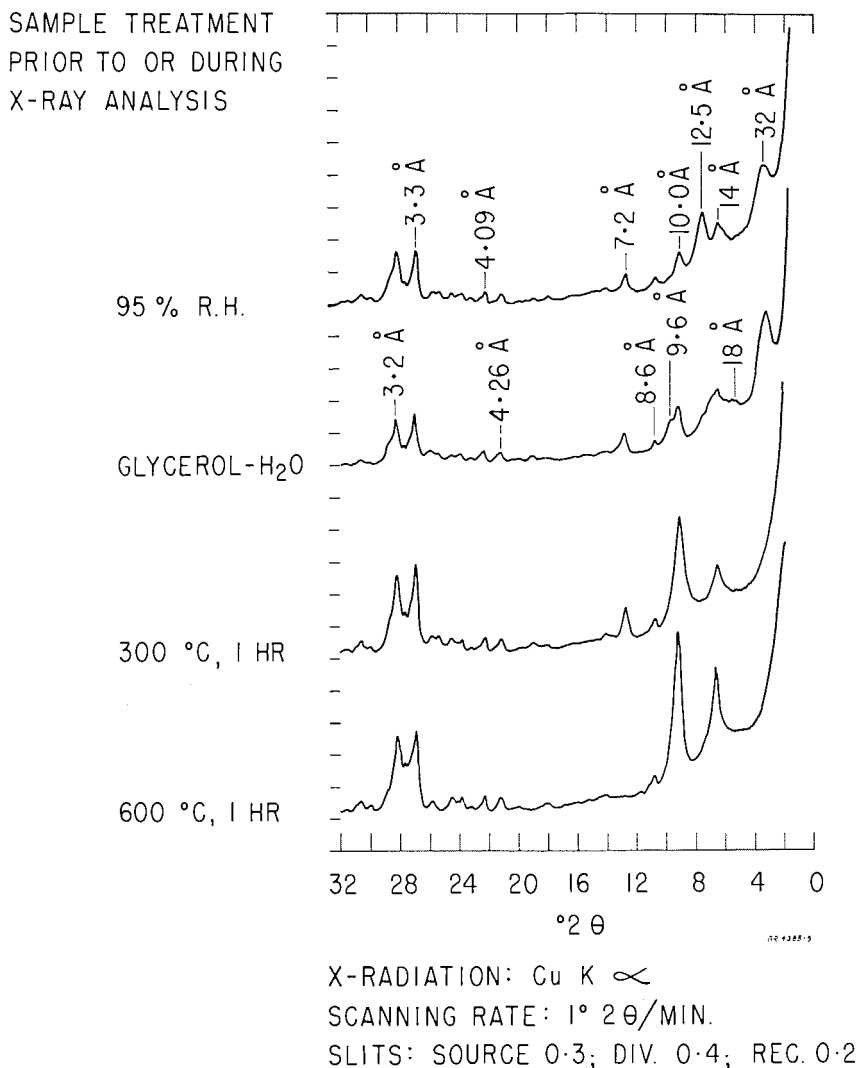
FIG. 1. X-ray diffractograms of sample A . 2-0.2 \mu m fraction.
