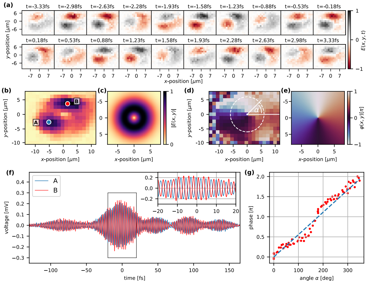
Fig. 3. Spatially resolved measurements of OAM beams: (a) Field amplitudes as a function of space and time, normalized to unity. (b) Amplitude of the measured current modulation induced by the OAM beam together with the expected shape for the theoretical Laguerre–Gaussian beam shown in (c). Deviations between experimental data and the simple OAM profile can be attributed to astigmatism in the focusing optics as well as to a non-Gaussian mode shape that has been used for the vortex generation. (d) The extracted phase at each point in the sampled plane exhibits a helical profile as theoretically shown in (e). The angle \alpha defines a polar coordinate system. (f) Field sampling with nanoTIPtOE at the points A and B at opposite sides of the focus, indicated in (b). (g) The phase for each point within the dashed circle in (d) (red dots) shows a linear trend with \alpha (dashed blue line). The raw data used for the plots in (a), (b), (d), and (g) can be seen in Figure S1 of Supplement 1. To generate the plot in (f), a Fourier filter from 0.1 to 1 PHz has been applied in order to remove nonlinear distortions.
