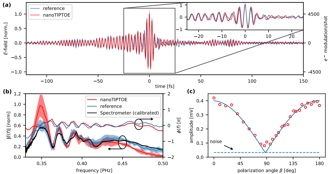
Fig. 2. Field measurement using nanoTIPTOE: (a) Average and standard deviation of five nanoTIPTOE field measurements in the center of the laser focus together with a reference obtained using TIPTOE in gas. The standard deviation is of the order of the linewidth. We corrected the data for a small offset by removing frequency components below 0.01 PHz. The enhanced intensities were (7.2 \pm 0.9) \times 10^{13} \frac{\text{W}}{\text{cm}^2} and (4.6 \pm 0.6) \times 10^{12} \frac{\text{W}}{\text{cm}^2} for the pump and signal beam in the nanoTIPTOE regime, respectively. The second axis indicates the current modulation in the nanoTIPTOE regime. The excellent agreement of nanoTIPTOE and standard TIPTOE can be seen in the inset. (b) Spectral amplitudes with error bar and spectral phase, obtained via a Fourier transform of the data in (a) as well as the calibrated spectrum recorded with a spectrometer. (c) Detected amplitudes depending on the polarization angle of the linearly polarized signal beam (red dots). As expected, the signal scales proportional to |\cos(\beta)| . The pump polarization remained the same.
