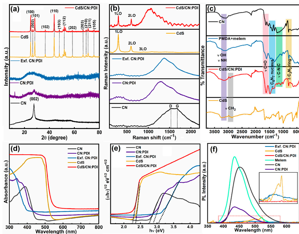
Figure 4. (a) XRD diffraction pattern, (b) Raman spectra, (c) FTIR (d) DR-UV-Vis spectra (e) Tauc plot and (f) steady-state PL spectra of CN (black), CN:PDI (violet), Exf. CN:PDI (blue), CdS (yellow) and CdS/CN:PDI (red).
