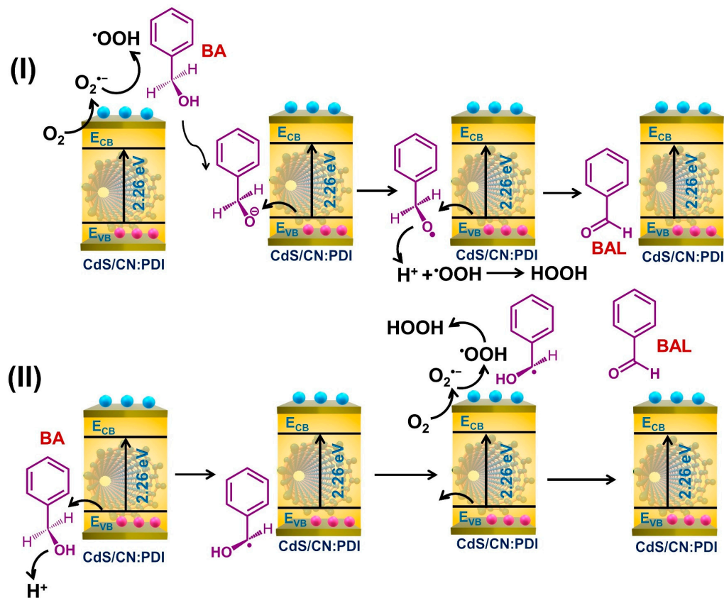
Figure 7. Mechanism of photo-oxidation of benzyl alcohol to benzaldehyde using CdS/CN:PDI via route I and route II.
