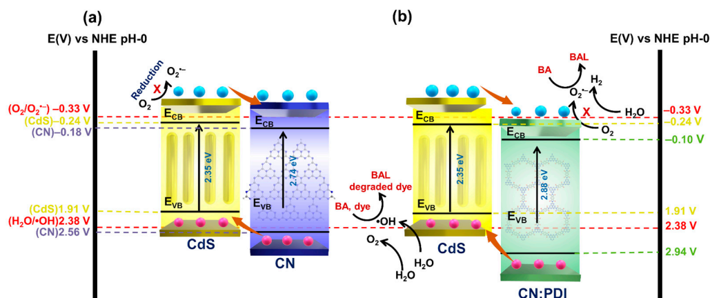
Figure 6. The band diagram displays the flow of electrons in (a) CdS/CN (b) CdS/CN:PDI.
