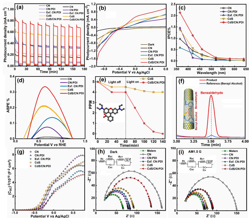
Figure 5. (a) Photocurrent vs. time ( i-t ) plot showing photoresponse during light On-Off cycle at +0.6 V under solar-simulated AM1.5G light irradiation without filter ( 100 \text{ mW cm}^{-2} ) with and AM1.5G light irradiation with a 420 nm cut-off filter. (b) LSV showing photocurrent density with respect to the applied voltage and (c) IPCE% vs. wavelength action spectra under 365, 420, 460, 520, 580, 640 nm wavelength LEDs ( 21.0 \text{ mW cm}^{-2} ). (d) ABPE% showing maximum photoconversion efficiency (PCE%) under AM1.5G light irradiation without filter ( 100 \text{ mW cm}^{-2} ) for CN, CN:PDI, Exf. CN:PDI, CdS, CdS/CN:PDI. (e) Photocatalytic degradation of RhB using CdS (yellow), CdS/CN:PDI (red) under AM1.5G light, (f) HPLC chromatogram of pure BA (blue) and the reaction product of photooxidation of BA showing the peak of BAL (red) using CdS/CN:PDI as a catalyst. (g) Mott-Schottky plot showing flat band potential. (h) EIS Nyquist plot under dark and (i) under AM1.5G irradiation. Inset showing Randles equivalent circuit. All the measurements were performed in 0.1 \text{ M Na}_2\text{SO}_4 solution at a scan rate of 0.1 \text{ mV/s} . Color: CN (black), CN:PDI (violet), Exf. CN:PDI (blue), CdS (yellow), CdS/CN:PDI (red).
