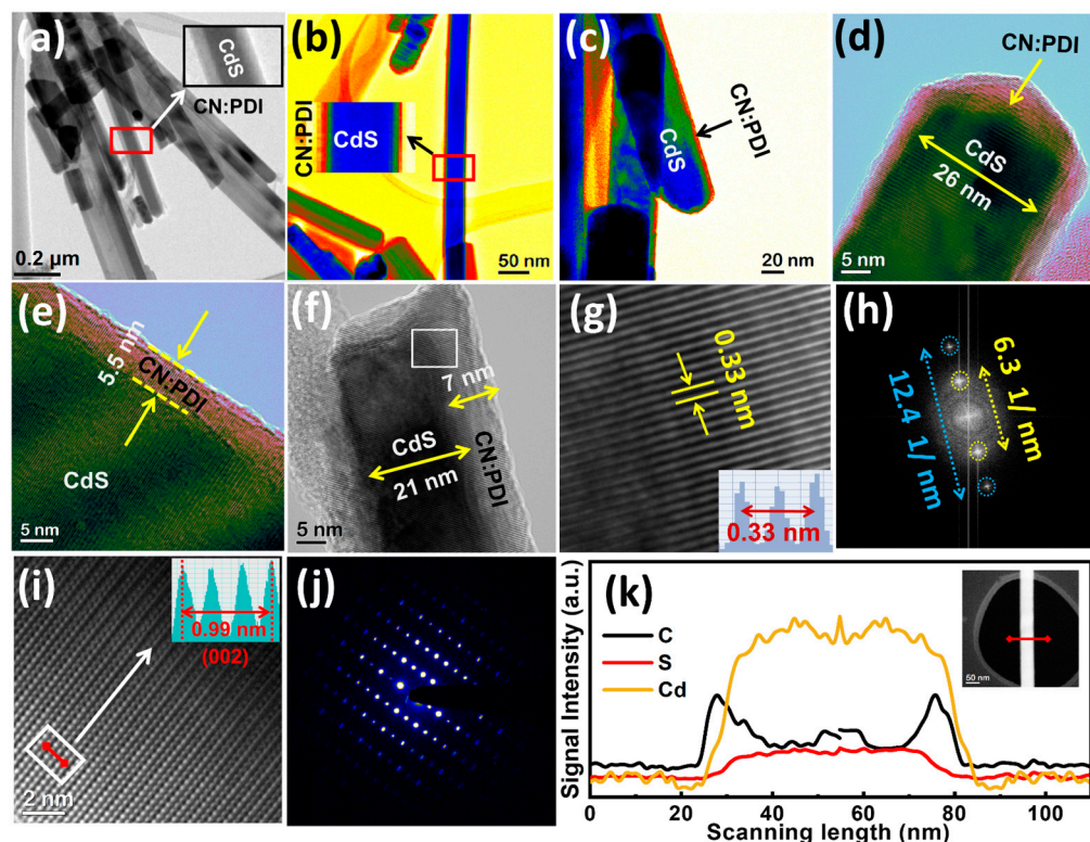
Figure 2. HR-TEM image of CdS/CN:PDI at (a) 0.2 \mu\text{m} (b) 50 nm (c) 20 nm scale bar showing CdS nanorod bundles with CN:PDI coating and HR-TEM images at (d–f) 5 nm scale bar showing the diameter of CdS and thickness of CN:PDI coating, (g) image of the selected area showing lattice fringes at the interface (h) FFT of the selected area (i) HR-TEM image at 2 nm scale bar showing the atomic column of CdS nanocrystal; inset showing d-spacing between atomic dots. (j) SAED pattern of CdS/CN:PDI and (k) electron energy-loss spectra (EELS) line scan on CN:PDI showing the distribution of Cd (yellow), S (red) and C (black) along the diameter of CdS/CN:PDI.
