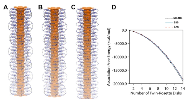
Fig. 4 Nanotubes made up of 7 quad-rosettes from 4a with SSS (A) and SAS (B) arrangements of the GAC units, and nanotube derived from NH-TBL (C), generated by the stacking of 14 twin-rosettes through simulation. Comparison of association free energies of nanotubes from 4a with SSS and SAS arrangements of the GAC units with increasing number of rosette stacks (up to 7 stacks), and of NH-TBL (up to 14 stacks) (D).
