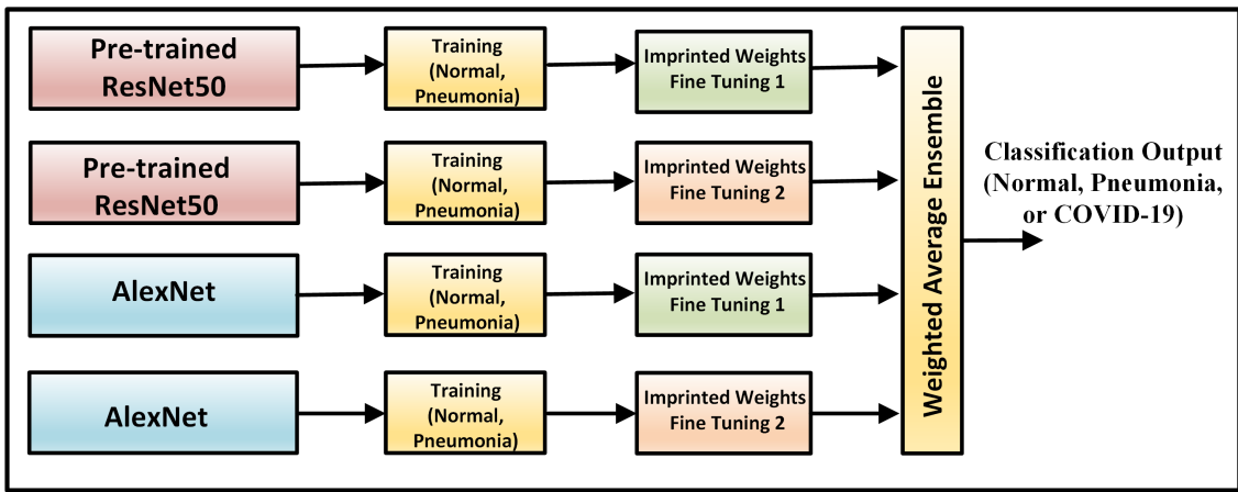
Fig. 1: The proposed ensemble approach integrating pre-trained deep CNNs with imprinted weights.
