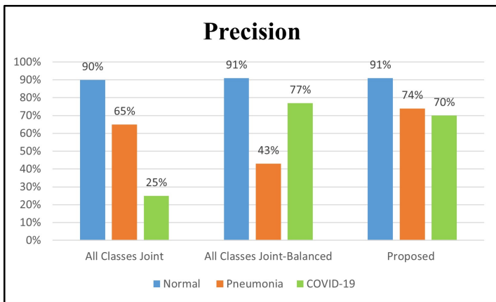
Fig. 3: The resulting performance in terms of precision.
