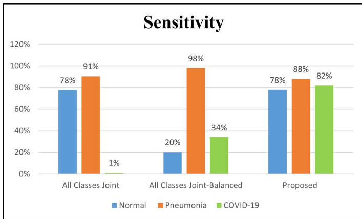
Fig. 2: The resulting performance in terms of sensitivity.
