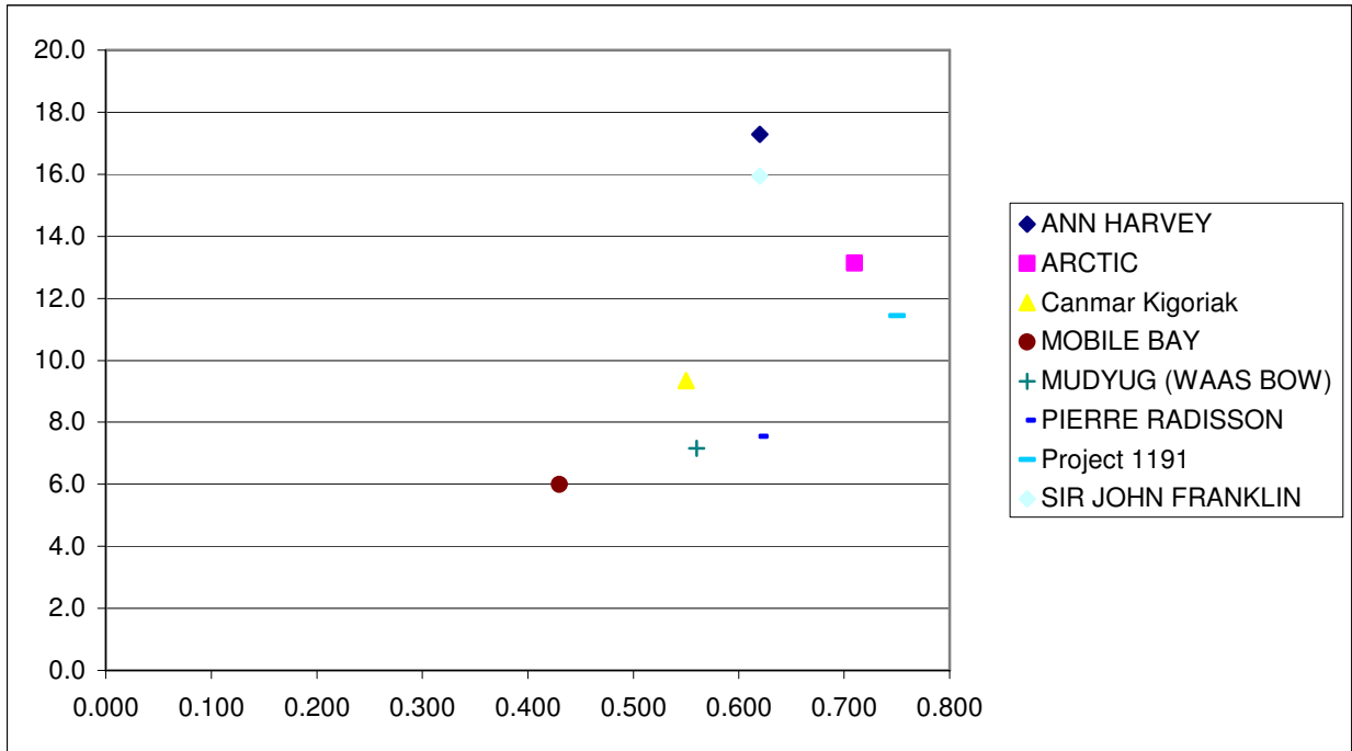
Figure 21: R/L vs. C B for Similar Test Conditions.
