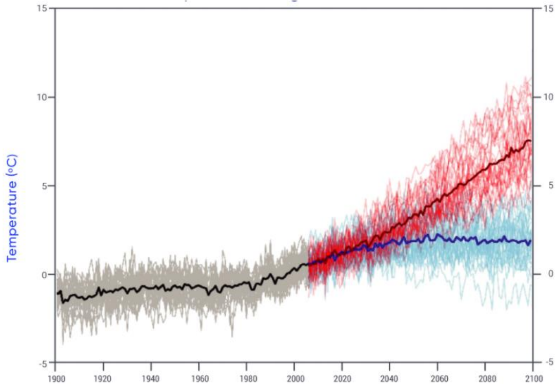
Figure 11: The temperature changes from 1900 to 2100 in Canada (Bush and Lemmen, 2019, Fig. 4.8). The grey trace is the observed temperature, and the blue and red lines are predictions for a low and a high emission scenario, respectively.
