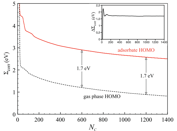
FIG. 2. (Color online) \Sigma_{\text{corr}} for the isolated (dashed line) molecule and molecular resonance (solid line) in the monolayer as a function of the number of conduction bands used in the evaluation of \hat{\Sigma} . Although the absolute value of these terms converge slowly, by N_c = 600 their difference \Delta\Sigma_{\text{corr}} (inset) has stabilized to 1.7 eV, attributable to nonlocal static correlations from the metal substrate. The nonlinear behavior of \Sigma_{\text{corr}}(N_c) for N_c < 200 reflects the character of low-energy conduction bands, which are highly system specific.
