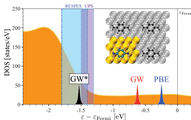
FIG. 1. (Color online) Electronic density of states (DOS) of 1,4-benzenediamine (BDA) above the Au(111) atop site. The inset shows the geometry of the 4 \times 4 supercell in color and periodic images in gray. The position of the highest occupied molecular orbital within DFT is -0.25 eV below the Fermi level. G_0W_0 (this work) differs from the experimental measurement by 0.8 eV. The source of this discrepancy is twofold: a 0.7 eV underestimate of the gas phase ionization energy (IE), and a 0.2 eV overestimate of the Au work function. Accounting for these errors with a post hoc correction, i.e., a rigid shift, produces a value ( GW^* ) in excellent agreement with experiment. Results from resonant and ultraviolet photoemission spectroscopy (RESPES/UPS) (Ref. 7) and their uncertainties are indicated by the shaded regions.
