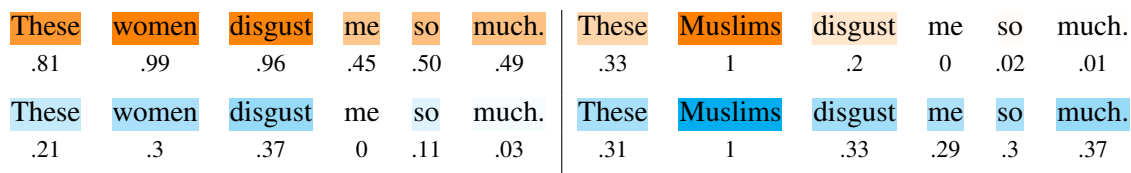
Figure 2: Visualization for necessity and sufficiency scores on an example HateCheck test case targeting women and Muslims for the classifier Founta2018-hate . Darker shades correspond to higher values.
