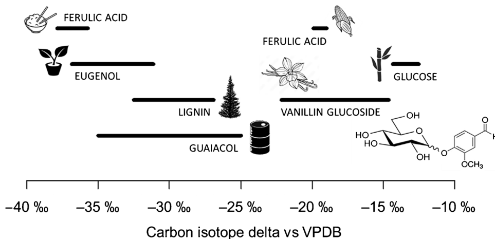
Fig. 1 Carbon isotope delta values of vanillin obtained from various sources
