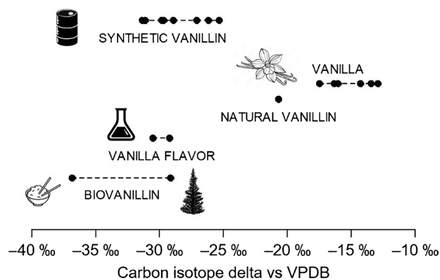
Fig. 2 Carbon isotope delta values for samples of vanillin and vanilla samples measured in this study
