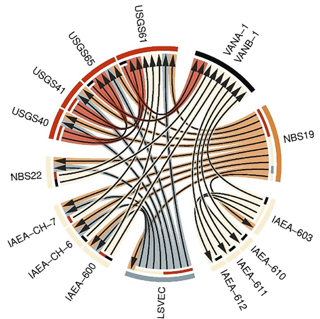
Fig. 3 Traceability pathway for carbon isotope delta values in VANA-1 and VANB-1
