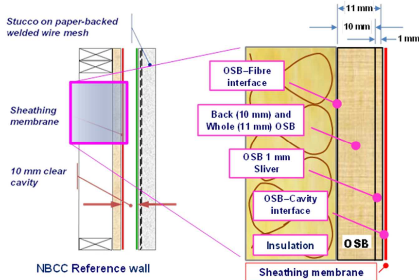
Figure 7 – Locations of interest within wall assemblies in assessing relative performance
