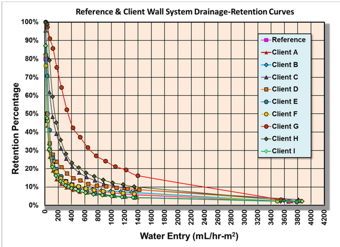
Figure 4 – Reference and Client wall system Drainage-Retention Curves
