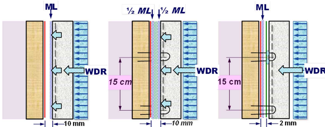
Figure 6 – Illustration of moisture load distribution within drainage cavity
