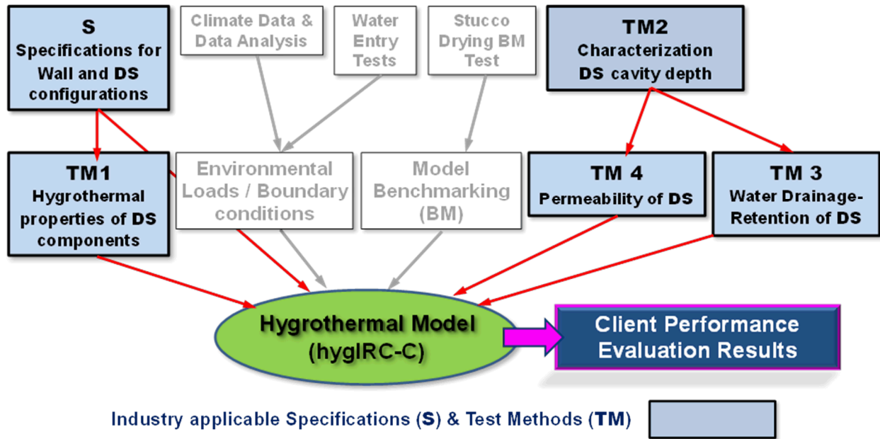
Figure 8 – Notional procedure and approach for drainage system (DS) product evaluation
