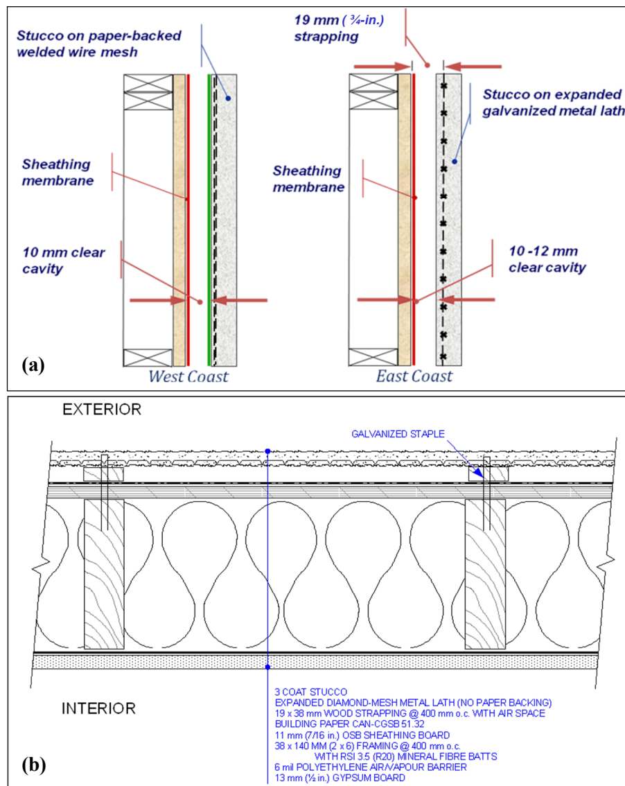
Figure 2 – (a) Vertical Sectional views of West and East coast solutions for stucco installation with capillary break; (b) Horizontal sectional view of East coast solution
