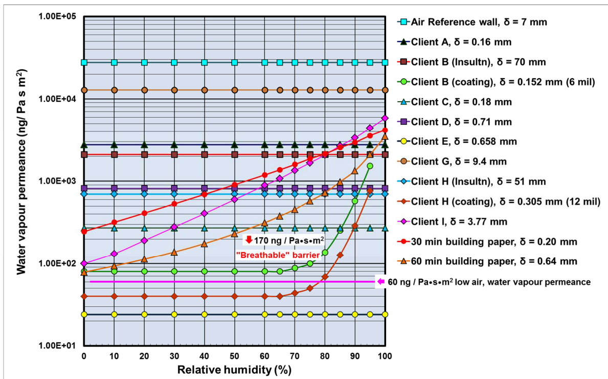
Figure 3 – Water vapour permeance of sheathing membranes as a function of RH used in respective Client drainage systems; \delta = thickness of membrane or insulation product
