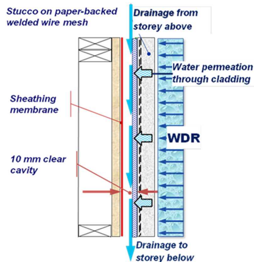
Figure 5 - Moisture loads within drainage cavities at given storey height
