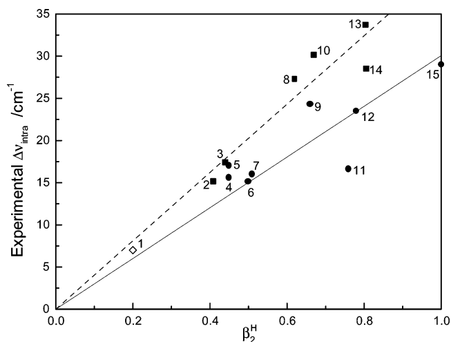
Figure 5. Plot of experimental \Delta\nu_{\text{intra}} values for catechol/HBA complexes versus \beta_2^{\text{H}} . Oxygen atom acceptor bases, ●, solid line; nitrogen atom acceptor bases, ■, dashed line and mesitylene, ◇ (not included in either fitting). The HBAs are numbered as in Table 2. The lines have been forced through (0,0).
