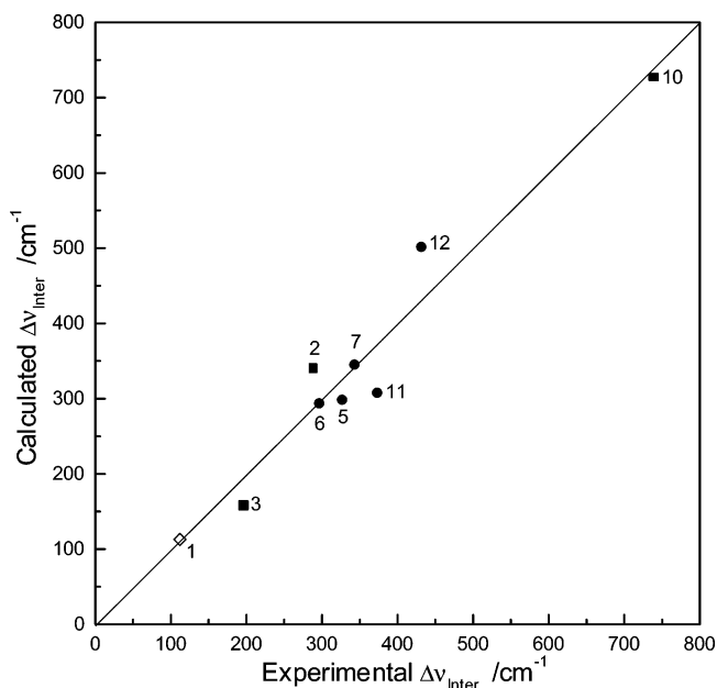
Figure 4. Plot of calculated versus experimental \Delta\nu_{\text{inter}} values for catechol/HBA complexes. Oxygen atom acceptor bases, ●; nitrogen atom acceptor bases, ■ and mesitylene, ◇. The HBAs are numbered as in Table 2. The straight line has a slope of 1.0.
