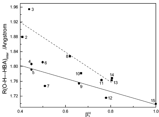
Figure 7. Plot of intermolecular HB length, R(\text{O–H} \cdots \text{HBA})_{\text{inter}} , for catechol/HBA complexes versus \beta_2^{\text{H}} . Oxygen atom acceptor bases, ●, solid line and nitrogen atom acceptor bases, ■, dashed line. The HBA's are numbered as in Table 2.
