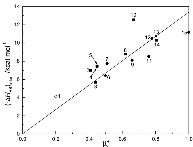
Figure 6. Plot of calculated hydrogen bond enthalpies for catechol/HBA complexes versus \beta_2^{\text{H}} . Oxygen atom acceptor bases, ●; nitrogen atom acceptor bases, ■ and mesitylene, ◇. The HBA's are numbered as in Table 2. The straight line has been forced through (0,0).
