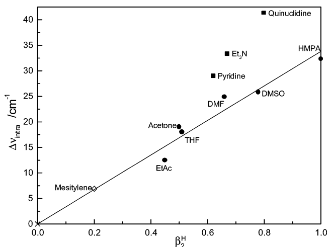
Figure 1. Plot of \Delta\nu_{\text{intra}} versus \beta_2^{\text{H}} for 3,5-di- tert -butylcatechol complexed with various oxygen (●) and nitrogen (■) bases. The straight line is the best fit to all of the data except those marked with ■, and is taken from ref 1. The fit is forced through (0,0).
