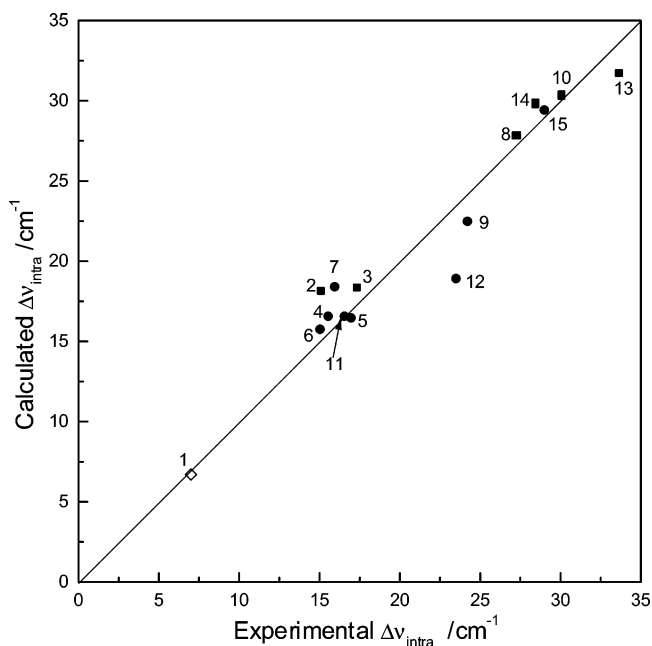
Figure 3. Plot of calculated versus experimental \Delta\nu_{\text{intra}} values for catechol/HBA complexes. Oxygen atom acceptor bases, ●; nitrogen atom acceptor bases, ■; mesitylene, ◇. The HBAs are numbered as in Table 2. The straight line drawn in this Figure has a slope of 1.0.
