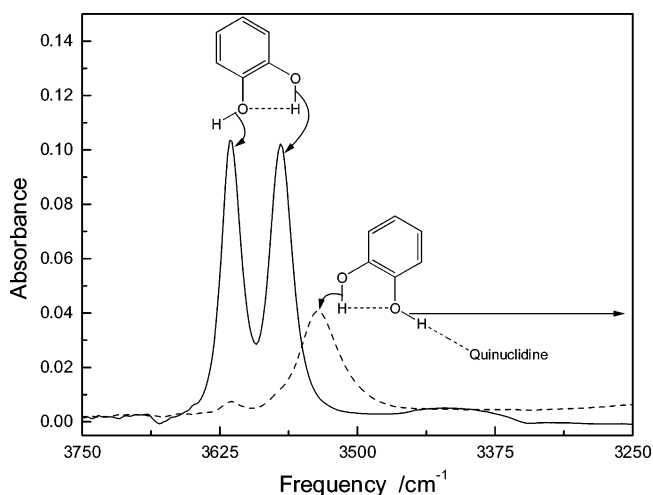
Figure 2. FT-IR spectra of catechol in \text{CCl}_4 (solid line) and catechol complexed with quinuclidine (dashed line). The origins of the bands are indicated.
