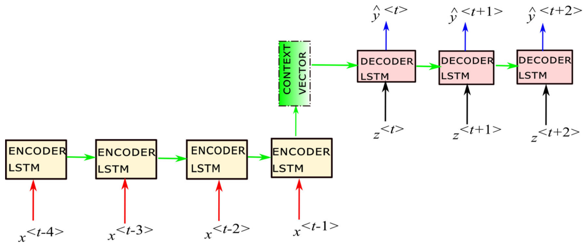
Fig. 5 A sample schematic representation of encoder-decoder LSTM architecture, with reduced feature space. Here, x^{<t-i>} is the vector containing input features (i.e., past meteorological and hydrological states and geophysical features) at the i th lag time, \hat{y}^{<t+j>} is the
