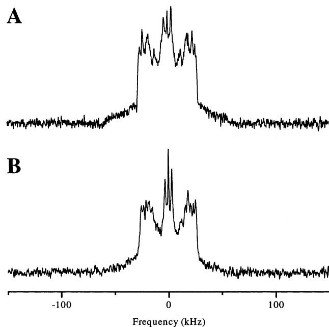
Figure 6. ^2\text{H} NMR spectra of 50/50 PA- d_{31} /chol mixture at pH 8.8, at (A) 30 and (B) 60 °C.
