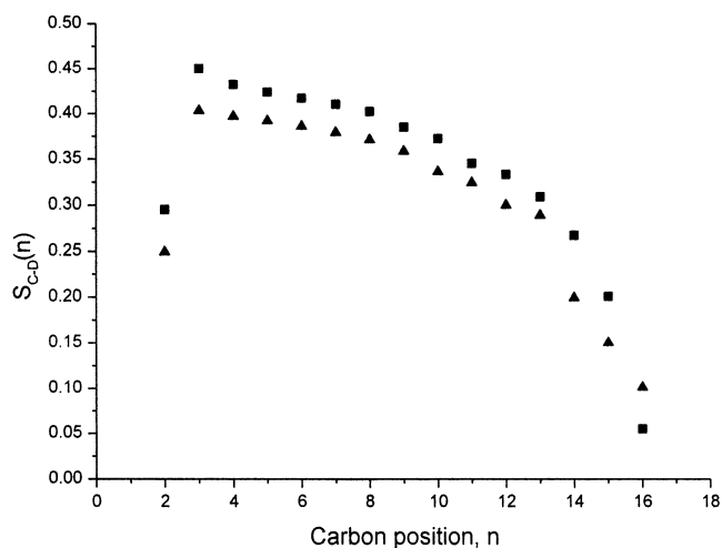
Figure 7. Orientational order profile for the 50/50 PA- d_{31} /chol mixture at pH 8.8 and T = 60 °C (■). For comparison purposes, the order profile for the same system at pH 5.5 and T = 55 °C (▲) is shown (reprinted with permission from ref 11. Copyright 2001 American Chemical Society).
