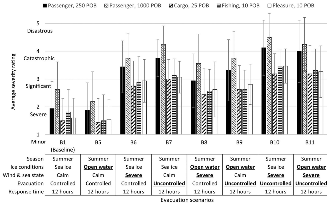
Figure 16. Average life-safety consequence severity, summer scenarios (Browne et al. 2021).
