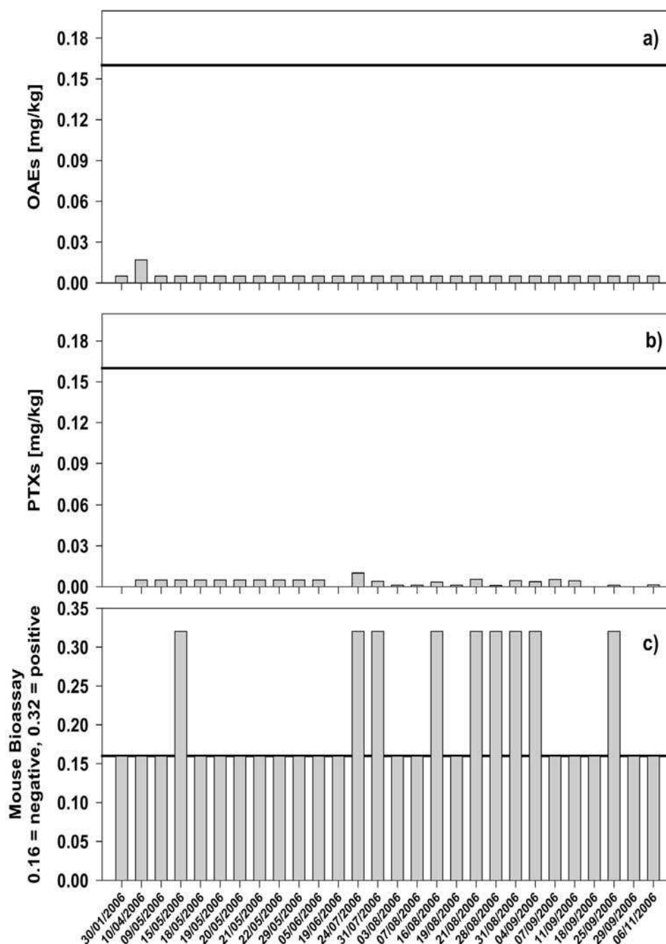
FIGURE 8 Temporal trends of OA-group toxins, PTX-group toxins and MBA results in oysters ( C. gigas ) from Arcachon, Bay of Biscay, French Atlantic Coast
