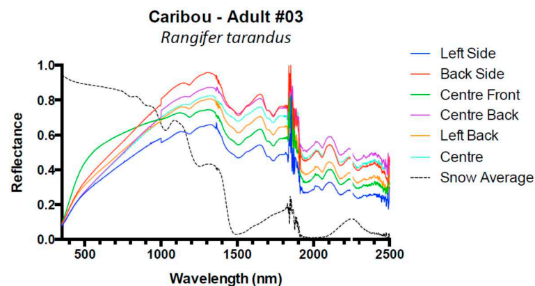
Figure A6. Spectral reflectance measurement of snow average along with measurements of various locations from the pelt 03 Adult Caribou. These data were used to calculate an average spectral reflectance for the pelt.
