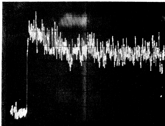
FIG. 9. Time dependence of R_1(\pm \frac{3}{2}) fluorescence on suddenly turning on laser to excite R_1(\pm \frac{1}{2}) line. Time scale 0.1 sec/cm. Zero applied field.
