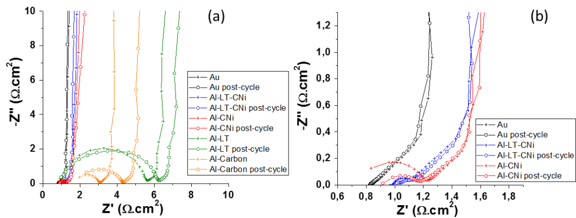
Figure S2 : (a) Nyquist Plots of supercapacitor cells assembled with different current collectors before and after 10,000 cycles ; (b) Zoom on the 0-2 Ω.cm 2 region.
