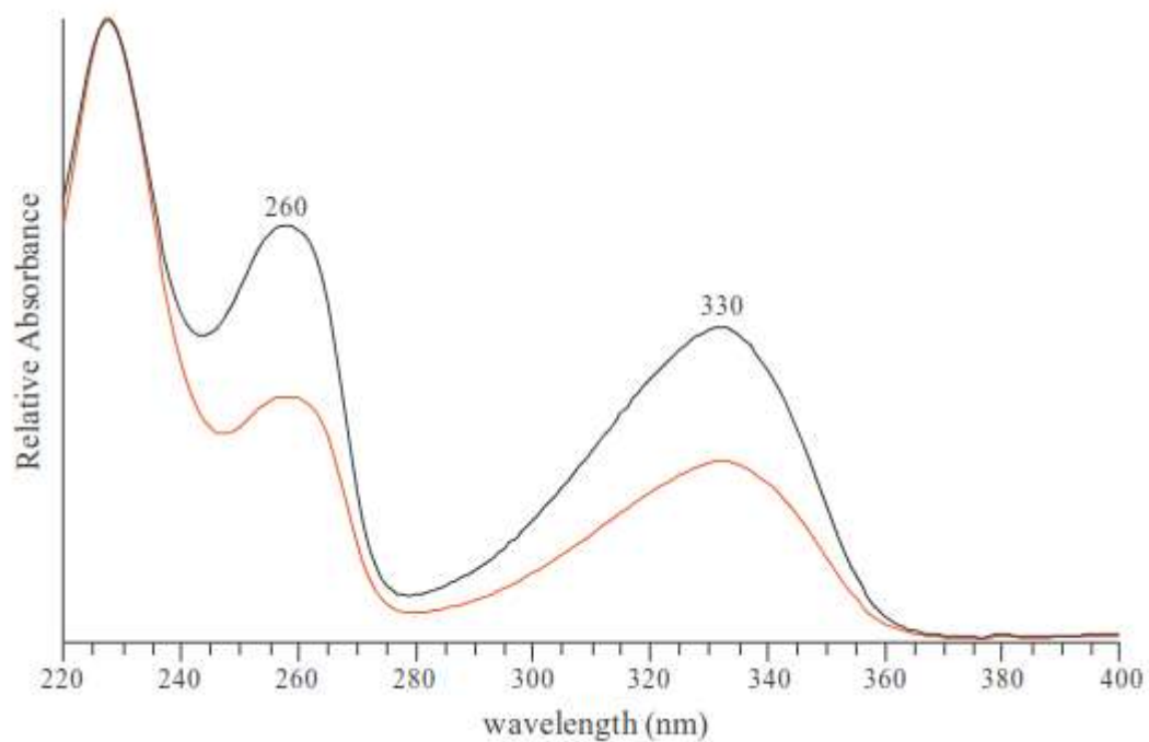
Figure S2. Normalized UV absorbance spectra for janthitrems C, 3 , (red) and D, 4 , (black) obtained with a PDA during HPLC analysis of fractions from P. janthinellum extracts.
