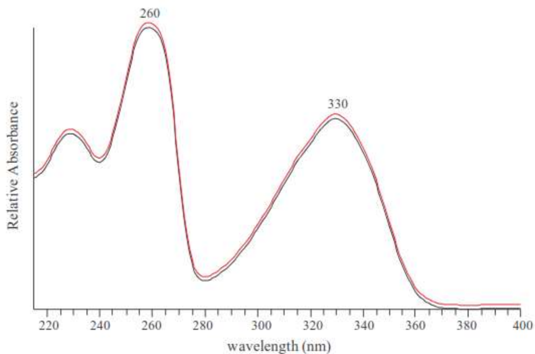
Figure S1. Normalized UV absorbance spectra for janthitrems A, 1 , (red) and B, 2 , (black) obtained with a PDA during HPLC analysis of fractions from P. janthinellum extracts.
