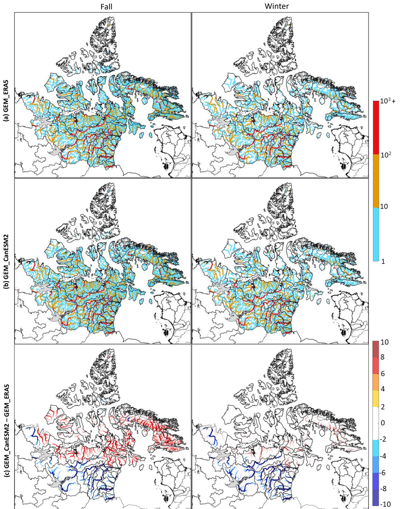
Figure S1: Spatial plots of mean fall and winter flows ( \text{m}^3/\text{s} ) for (a) GEM_ERA5 and (b) GEM_CanESM2 and (c) their differences for the 2001–2020 period.
