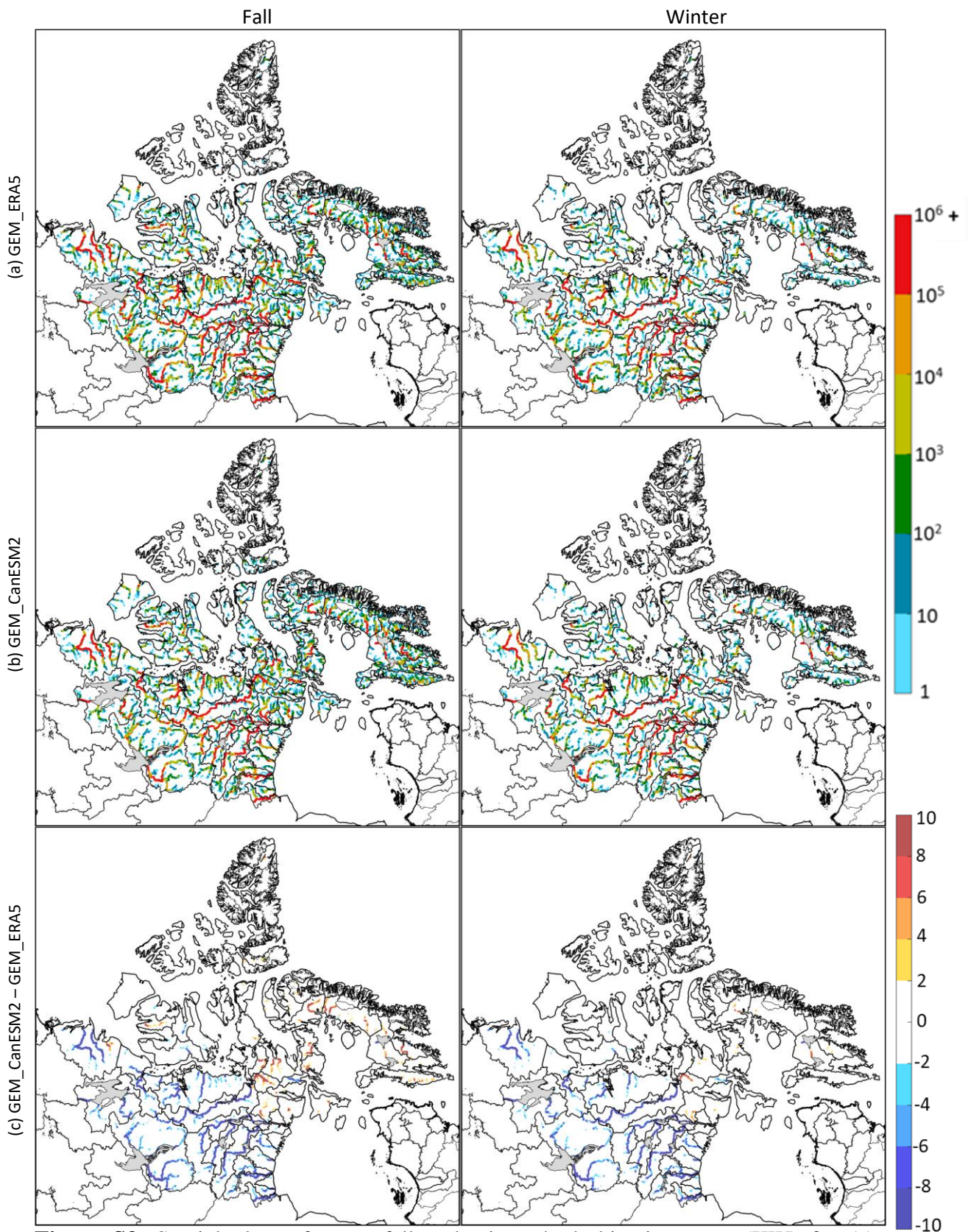
Figure S3: Spatial plots of mean fall and winter hydrokinetic power (KW) for (a) GEM_ERA5 and (b) GEM_CanESM2 and (c) their differences for the 2001–2020 period.
