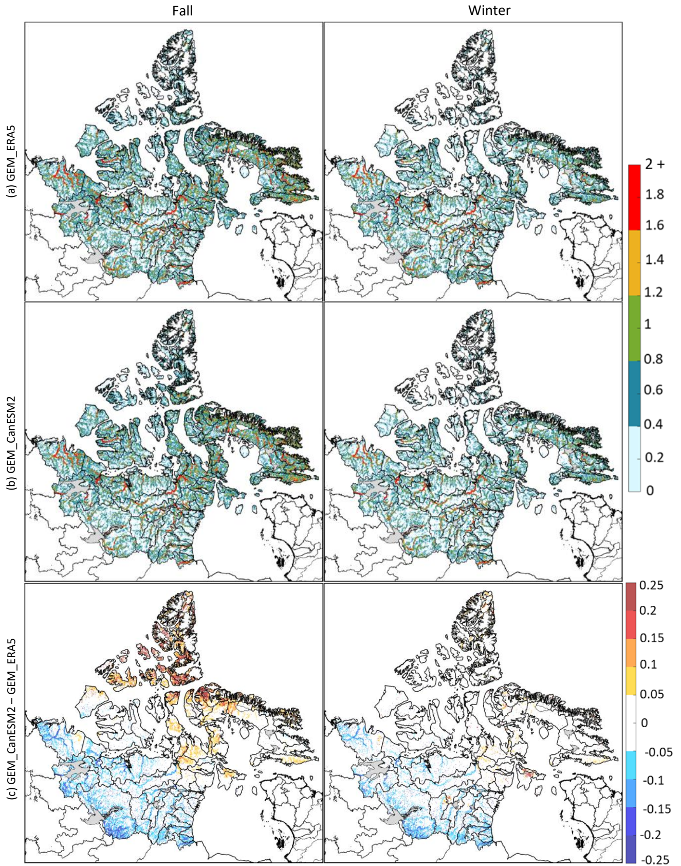
Figure S2: Spatial plots of mean fall and winter flow velocities (m/s) for (a) GEM_ERA5 and (b) GEM_CanESM2 and (c) their differences for the 2001–2020 period.
