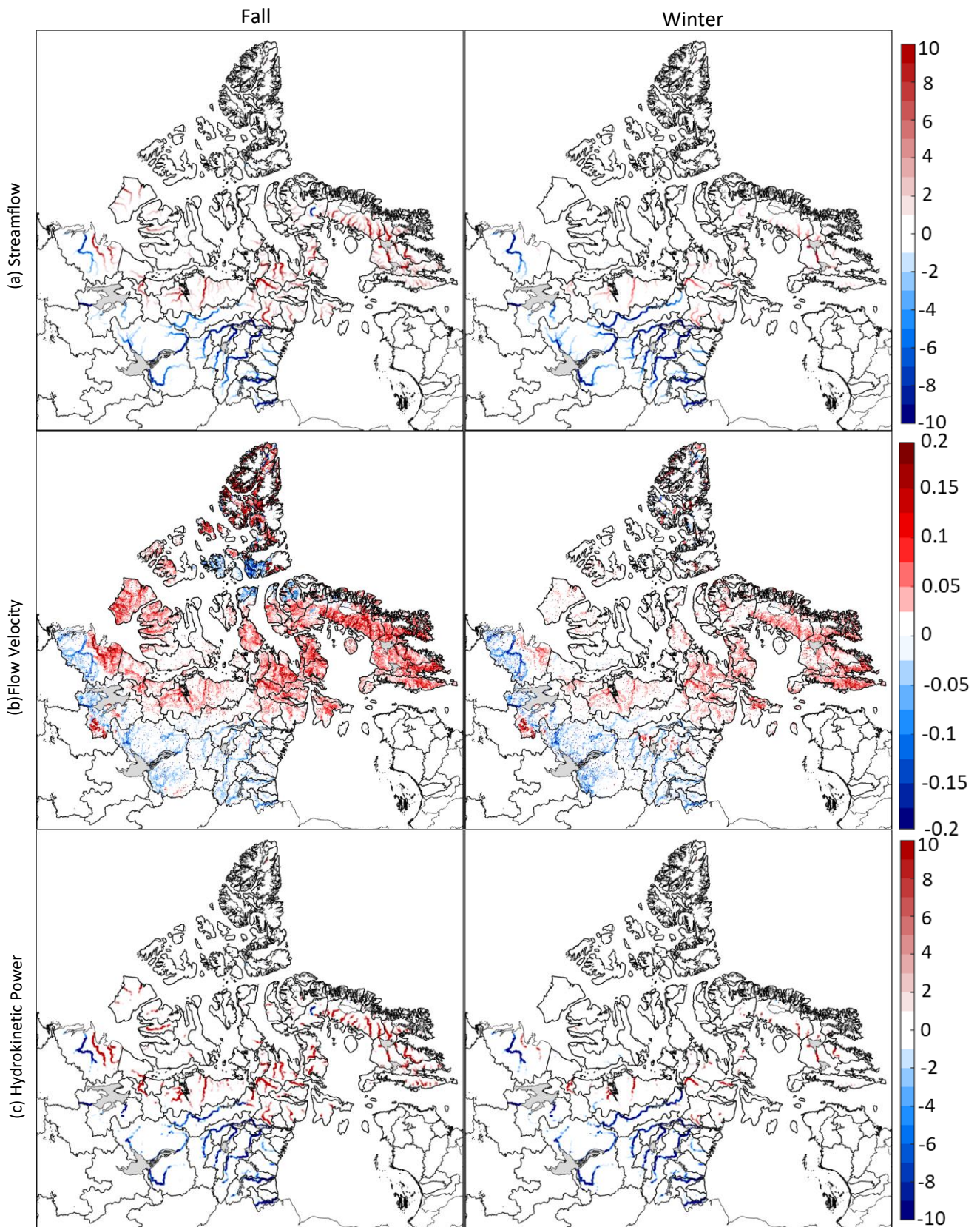
Figure S4: Projected changes to mean fall and winter (a) streamflow ( \text{m}^3/\text{s} ) (b) flow velocity ( \text{m}/\text{s} ) and (c) hydrokinetic power (KW) for the 2021–2040 period with respect to 2001–2020 period.
