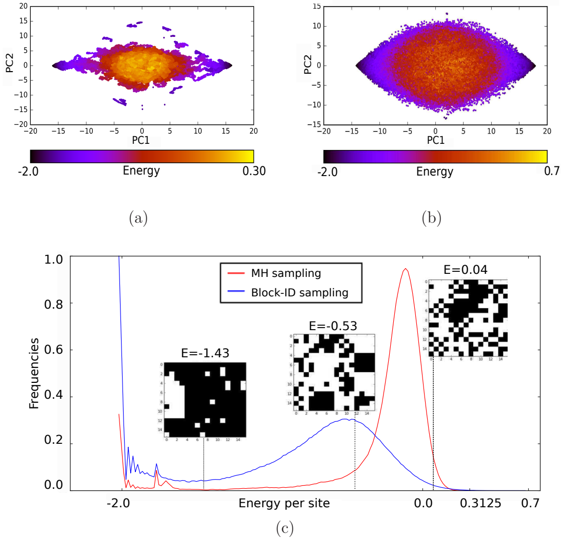
Figure 10: (a-b) PCA view and (c) energy distributions of datasets generated by Metropolis-MC and block-ID sampling techniques for 16 \times 16 Ising model. Both datasets consist of 4,000,000 samples.
