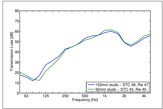
Figure 7. Influence of stud depth. Decreasing the stud depth without changing other parameters degrades the sound insulation performance, because the smaller air gap between the two sides leads to an upward shift of the mass-spring-mass resonance frequency.
