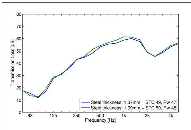
Figure 8. Influence of steel thickness. The steel thickness was found to be of minor importance in this study. However, light gauge walls will show different behaviour in terms of sound insulation.
