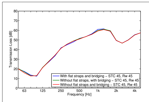
Figure 9. Influence of flat straps and bridging channel. The flat straps and bridging channels do not have a measurable influence on the direct sound insulation of the walls. They may however contribute to flanking sound transmission.
