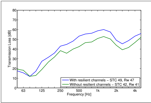
Figure 5. Influence of resilient channels. Resilient channels are among the most effective devices to improve sound insulation performance. The improvement is even higher for walls with more than one layer of gypsum board on each side.
