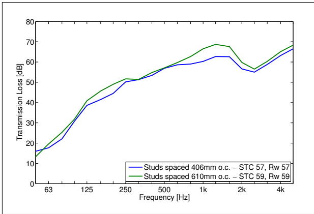
Figure 6. Influence of stud spacing. Increasing the stud spacing improves the sound insulation performance due to less structural connections between the two sides and due to decreased stiffness of the wall.
