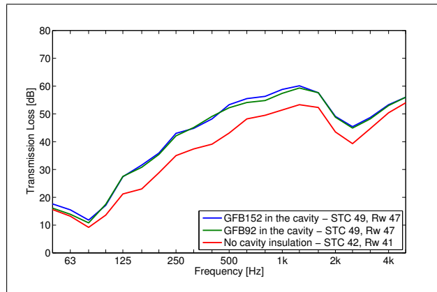
Figure 4. Influence of cavity insulation. Removing the cavity insulation from the reference assembly has a significant effect on the Sound Transmission Loss curve. The thickness of the insulation material tested here is of minor importance.
