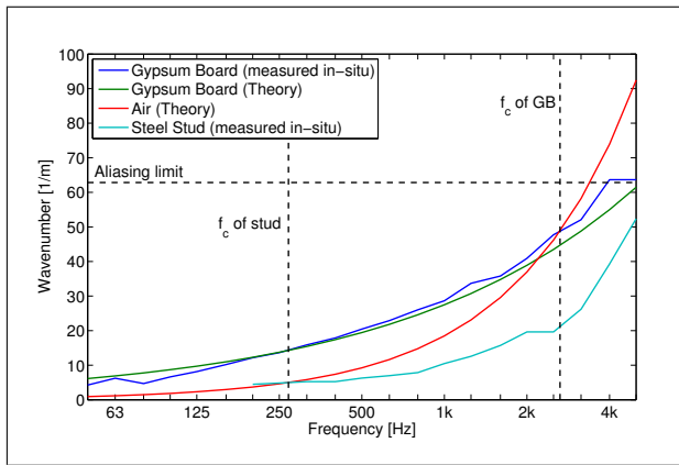
Figure 10. Wavenumbers measured on reference assembly. The cross-over points between the gypsum board/steel stud wavenumbers and the theoretical wavenumbers in air indicate the coincidence frequency of the gypsum board/steel stud, at and above which the gypsum board/steel stud radiates very efficiently.
