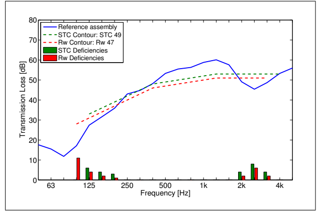
Figure 2. Sound Transmission Loss of reference assembly: G16_SS152(406)_GFB152_RC13(406)_G16
