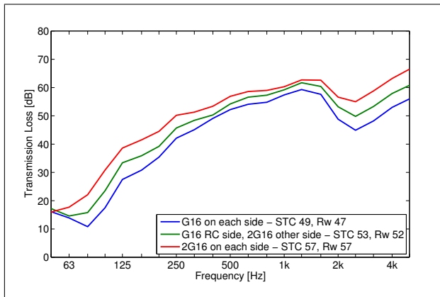
Figure 3. Influence of sheathing. For additional layers of gypsum board, the mass-spring-mass resonance shifts from the 80 Hz band into the 63 Hz band and further into the 50 Hz band.
