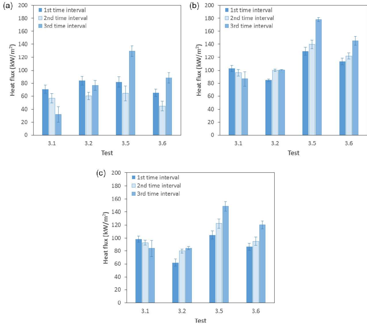
Figure 8: Time-averaged total heat flux to calorimeter, (a) top centre plane, C0, (b) bottom left plane, L180, (c) bottom right plane, R180
