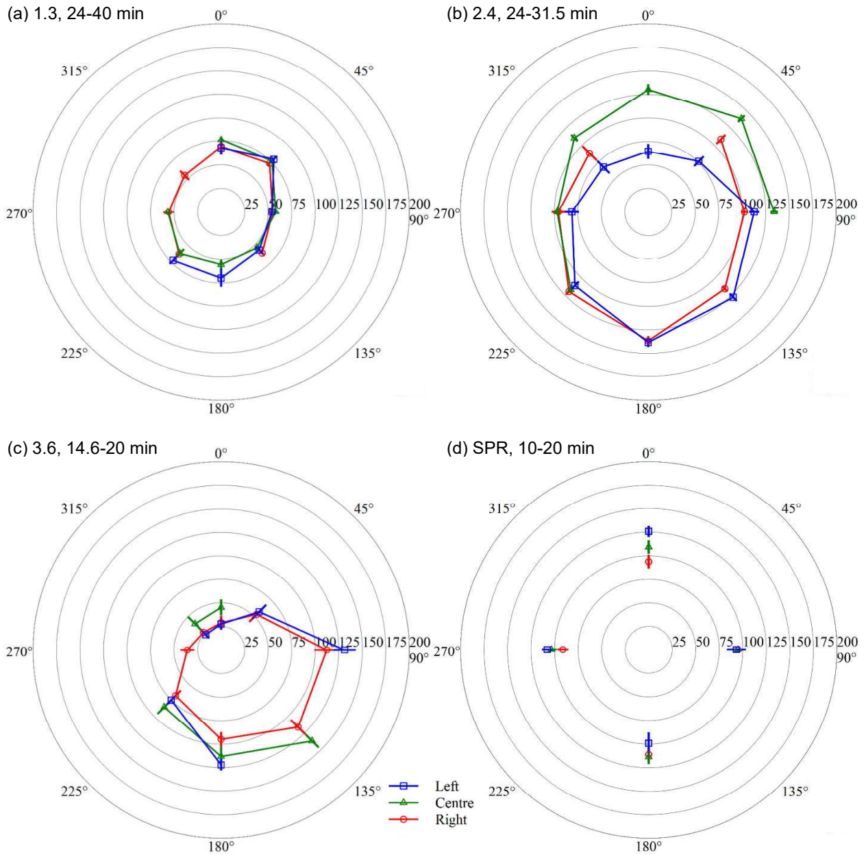
Figure 46: Selected plots of total heat flux ( \text{kW/m}^2 ) to calorimeter, for tests with calorimeter at 1 m height and 60^\circ\text{C} constant level fuel supply (SPR data from [8])
