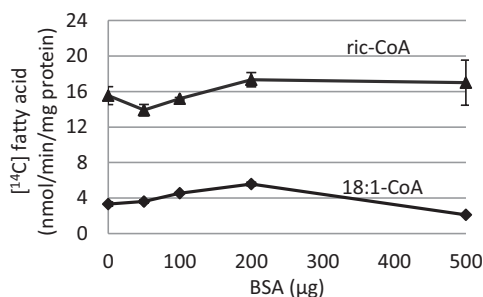
FIGURE 8. Effect of BSA on yeast microsomal acyl-CoA esterase activity toward [ 14 C]18:1-CoA and [ 14 C]ricinoleoyl-CoA in microsomal preparations of yeast ale1 microsomes transformed with empty vector. Incubations contained 20 μg of microsomal proteins and 5 nmol of acyl-CoA and additions of BSA as indicated in the figure in a total volume of 100 μl. Incubation time for [ 14 C]18:1-CoA was 10 min and for [ 14 C]ricinoleoyl-CoA (ric-CoA) 2 min. Experiments were performed in duplicate ±S.D.
