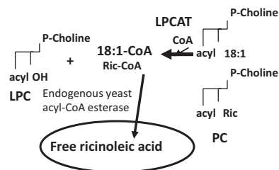
FIGURE 7. Main reactions in the metabolism of the mixture of ricinoleoyl-PC and oleoyl-PC with expressed AtLPCAT in yeast microsomes. Ricinoleoyl groups from PC are preferentially acylated to CoA over oleoyl groups to yield ricinoleoyl-CoA. The ricinoleoyl-CoA is then rapidly and preferentially hydrolyzed over oleoyl-CoA to free ricinoleic acid. The main products of LPCAT reversible reaction in these microsomes are thus oleoyl-CoA and free ricinoleic acid. Ric, ricinoleoyl.
